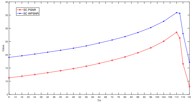
Fig. 5. PSNR and WPSNR curves of shadow images.
