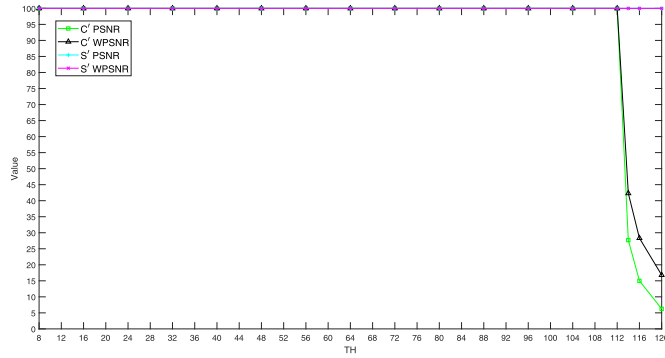
Fig. 6. PSNR and WPSNR curves of recovered cover images and the reconstructed secret image.
