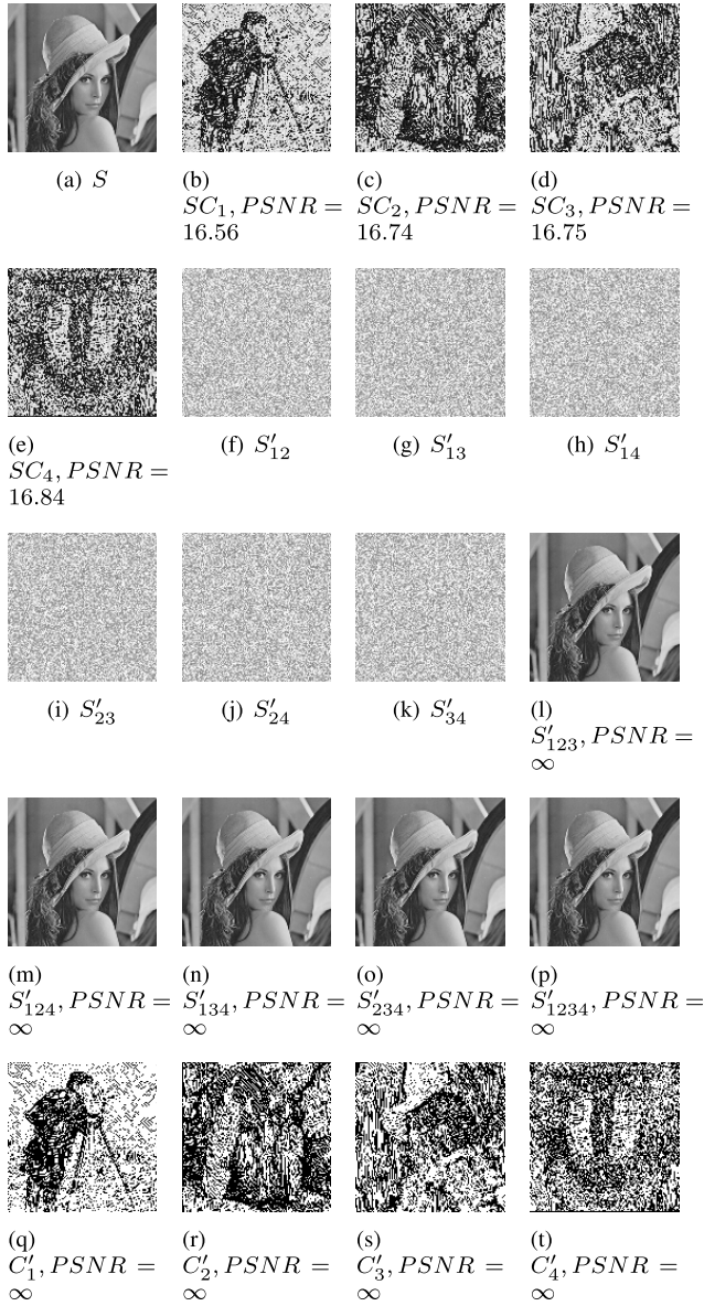
Fig. 3. Experimental results of the introduced (k, n) threshold RISS, where k = 3, n = 4, m_1 = 251, m_2 = 253, m_3 = 254, m_4 = 255, p = 131 and TH = 64 . (a) The grayscale secret image; (b) – (e) four grayscale comprehensible shares SC_1, SC_2, SC_3 and SC_4 ; (f) – (p) reconstructed grayscale secret images; (q) – (t) recovered binary cover images.
