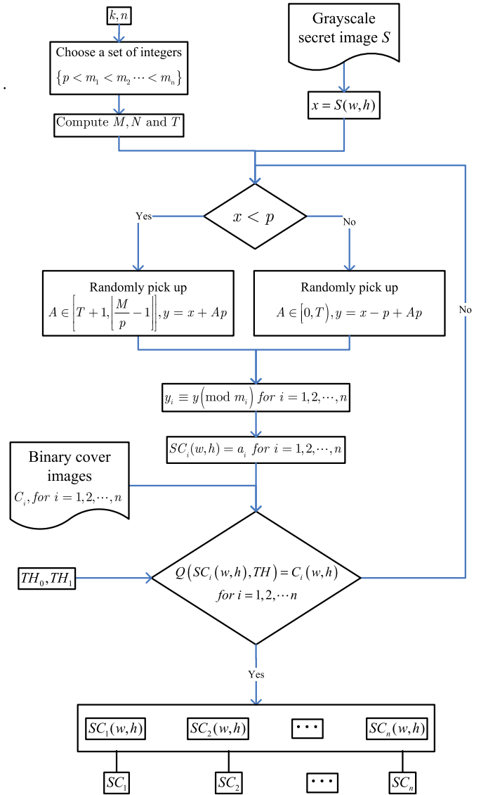
Fig. 1. Design idea of the proposed reversible image secret sharing algorithm.
