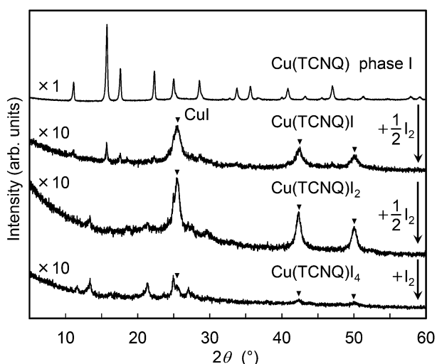
Fig. 5 Powder X-ray diffraction patterns of Cu(TCNQ)I n ( n = 1, 2, and 4 ) obtained by stepwise solid-state reactions of phase I Cu(TCNQ). Triangles indicate peaks for CuI.
