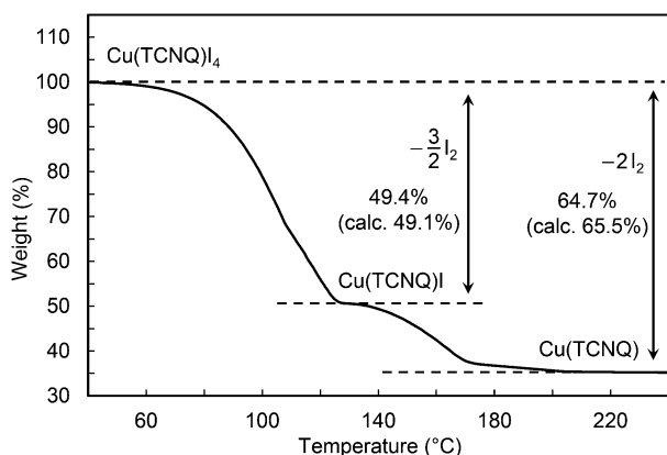
Fig. 4 Thermogravimetric traces of Cu(TCNQ)I 4 prepared by solid-state reactions of phase I Cu(TCNQ).
