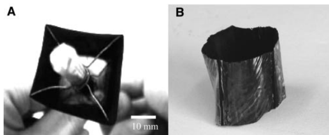
Fig. 4. (A) An end view of nanotubes wound onto a square wire former to cover it. (B) A wound nanotube covering after infiltration with polyvinyl chloride and removal of the former.
