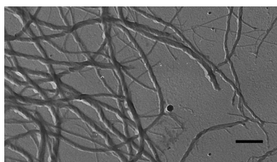
Fig. 3. Electron micrograph (TEM) of toluene gel of 1 ; the chiral fibers can be clearly seen (concentration, 1.8 mM; platinum shadow, 45°; scale bar, 500 nm).
