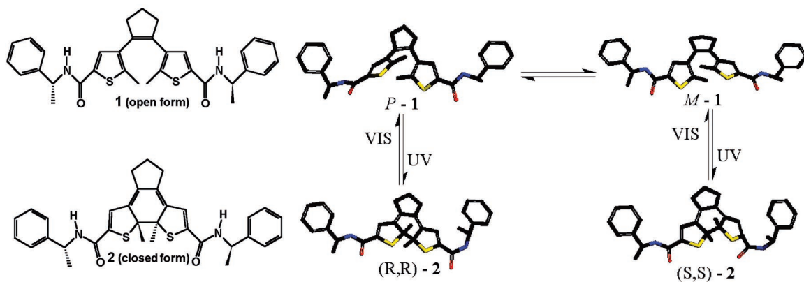
Fig. 1. Chiral switch 1 , which contains amide functionalities to induce aggregation by multiple hydrogen bonding, exists in the open form in two helical conformations P -1 and M -1 in rapid equilibrium. These can be transformed by irradiation into closed forms 2 . ( R,R )- 2 can only be obtained from P -1, and ( S,S )- 2 is exclusively formed from M -1. The two 1-phenylethylamine moieties continue to have the R configuration in either diastereomer of 2 . VIS, visible light.
