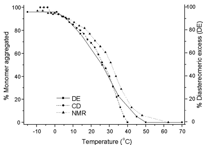
Fig. 4. Temperature dependency of the CD effect [wavelength ( \lambda ) = 320 nm], extent of aggregation ( ^1\text{H NMR} ), and diastereoselectivity of photochemical formation of 2 in toluene {the molar fraction aggregated is related to the CD effect by [\theta(\text{mdeg})_{\text{obs}}/\theta(\text{mdeg})_{\text{max}}] \times 100 }. The excellent correlation clearly indicates that these are related phenomena.
