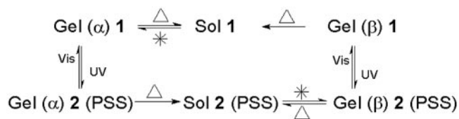
Fig. 5. Aggregation and switching processes and relation between different states. 1 , open form; 2 , closed form; UV, \lambda = 313 nm; visible (Vis), \lambda > 460 nm; *, cooling; \Delta , heating. Heat is required to irreversibly transform the unstable aggregates (from the \alpha to the \beta state and vice versa). Photochemical steps go with the retention of configuration; irradiation converts open form 1 and closed form 2 in a fully reversible manner.
