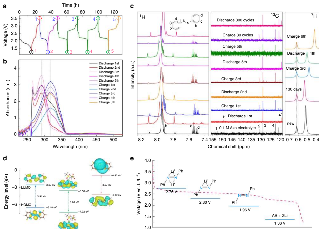
Fig. 6 Characterization of electrochemical reversibility and reaction mechanism. Charge and discharge profiles of 0.1 M AB electrolyte over time at the current density of 0.05 mA cm -2 ( a ) and corresponding UV-vis spectra recorded at different charge and discharge state ( b ). c 1 H, 13 C, and 7 Li NMR spectra of 0.1 M AB electrolyte measured at various selected charge and discharge cycles. d Optimized structure and calculated energy levels of AB, AB-LiTFSI, and Li 2 AB obtained from DFT simulations. e Comparison between the discharge voltage curve after the voltage evolution and predicted voltages of AB in different coordination configurations.
