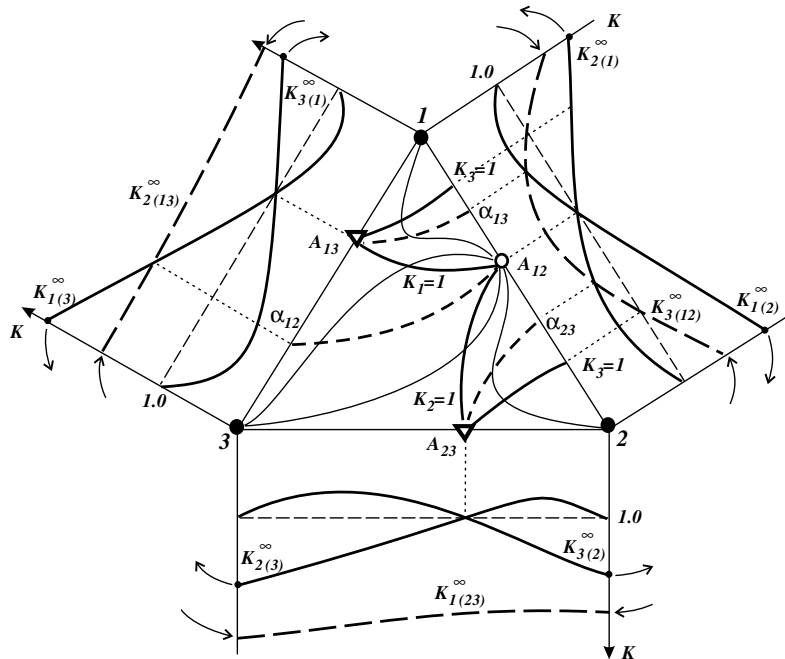
Fig. 49. Unidistribution and univolatility line diagram and sketch of the simple phase transformation line map for a mixture of Class 3.0–2.
