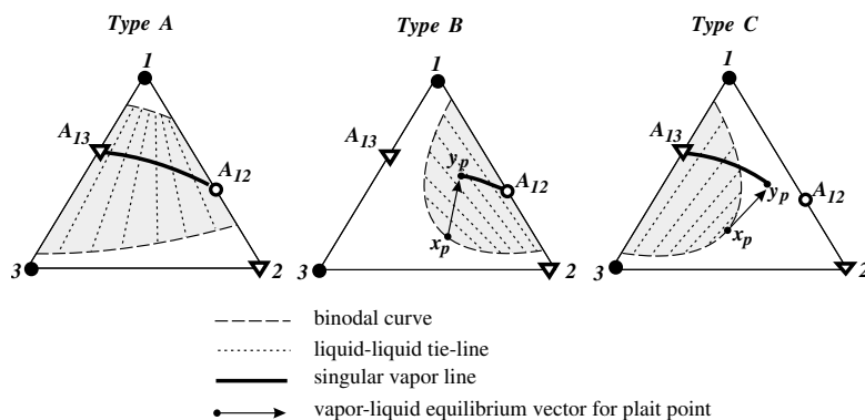
Fig. 18. Three possible types (A, B, C) of heterogeneity for a mixture with the boiling temperature structure of Serafimov's class 2.0–2b. The singular points are indicated by: (●) stable node, (○) unstable node, and (▽) saddle.
