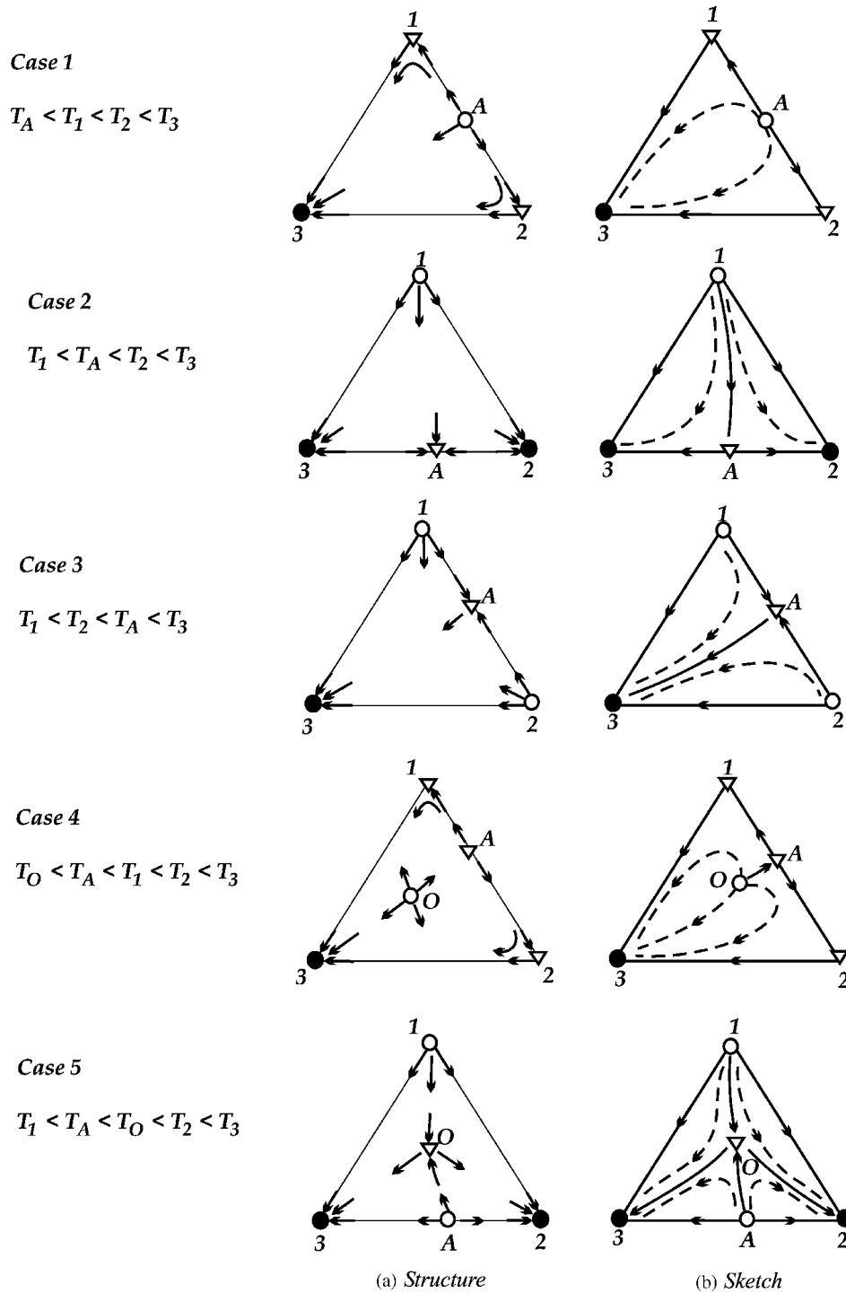
Fig. 10. Examples of qualitative residue curve map construction: (a) directions of residue curves near the singular points; (b) sketch of the residue curve diagram.
