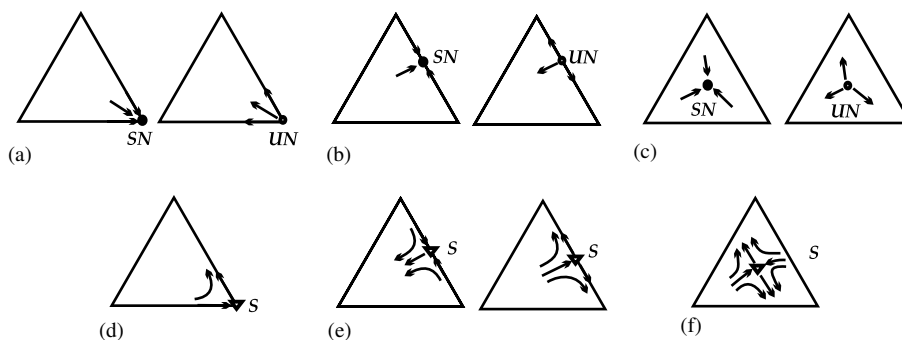
Fig. 8. Types of singular points for ternary mixtures indicated by • stable node (SN), ○ unstable node (UN), and ▽ saddle (S) (Zharov & Serafimov, 1975). Arrows point in the direction of increasing boiling temperature, and the letters (a, b, c, d, e, f) show the correspondence to Fig. 7.
