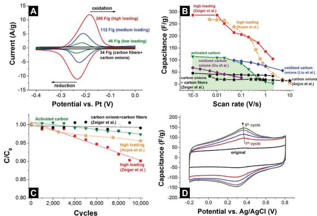
Fig. 14 (A) Cyclic voltammograms of carbon ion/carbon fiber composites loaded with different amounts of 9,10-phenanthrenequinones at 10 \text{ mV s}^{-1} scan rate. 129 (B) Rate handling data of different types of carbon onions, activated carbon, and carbon onions loaded with quinones or other functional groups. (C) Stability test using 10 000 cycles (CV) with activated carbon, carbon ion/carbon fiber composites, carbon onions and carbon ion/carbon fiber composites loaded with 9,10-phenanthrenequinones. (D) Cyclic voltammograms of carbon ions during electrochemical oxidation. All measurements were performed in 1 \text{ M H}_2\text{SO}_4 . 140 Zeiger et al. : nanodiamond-derived carbon ion/carbon fiber composites ( 1700^\circ\text{C} synthesis temperature) loaded with 9,10-phenanthrenequinones, three-electrode set-up, free-standing mats. 87 Anjos et al. : nanodiamond-derived carbon onions ( 1800^\circ\text{C} synthesis temperature), three-electrode set-up, dropcast on glassy carbon. 139 Gu et al. : nanodiamond-derived carbon onions ( 1800^\circ\text{C} synthesis temperature) oxidized with \text{H}_2\text{SO}_4/\text{HNO}_3 , two-electrode set-up, 1 \text{ M LiPF}_6 in PC, PTFE-bound electrodes (10 mass%). 124 Liu et al. : nanodiamond-derived carbon onions ( 1650^\circ\text{C} synthesis temperature with further oxidation in air at 400^\circ\text{C} ) electrochemically oxidized in 1 \text{ M H}_2\text{SO}_4 , three-electrode set-up, dropcast on glassy carbon. 140
