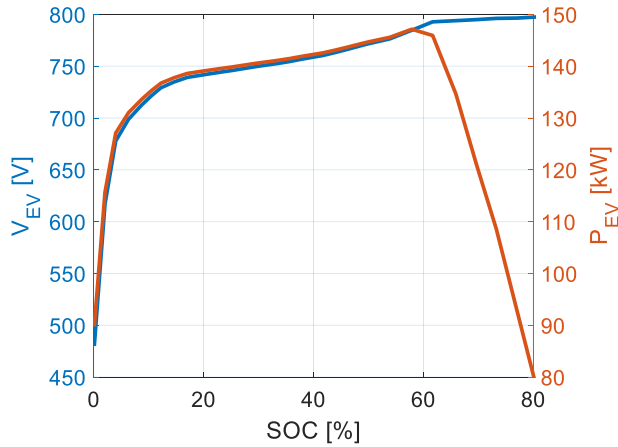
FIGURE 12. Voltage and power level of the EV through the charge.
