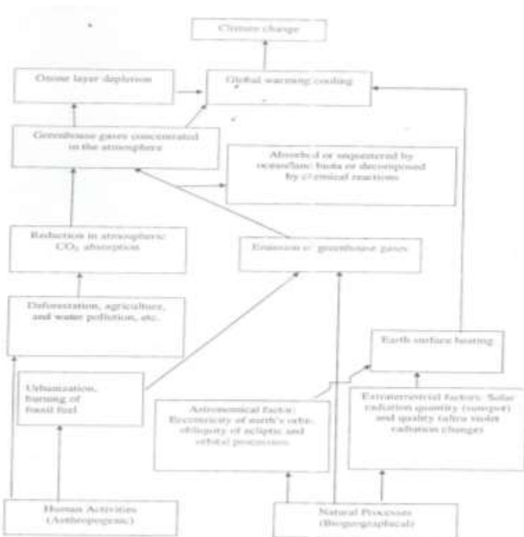
Figure 3. Causal factors of climate change. Source: Orlupe (2010).
