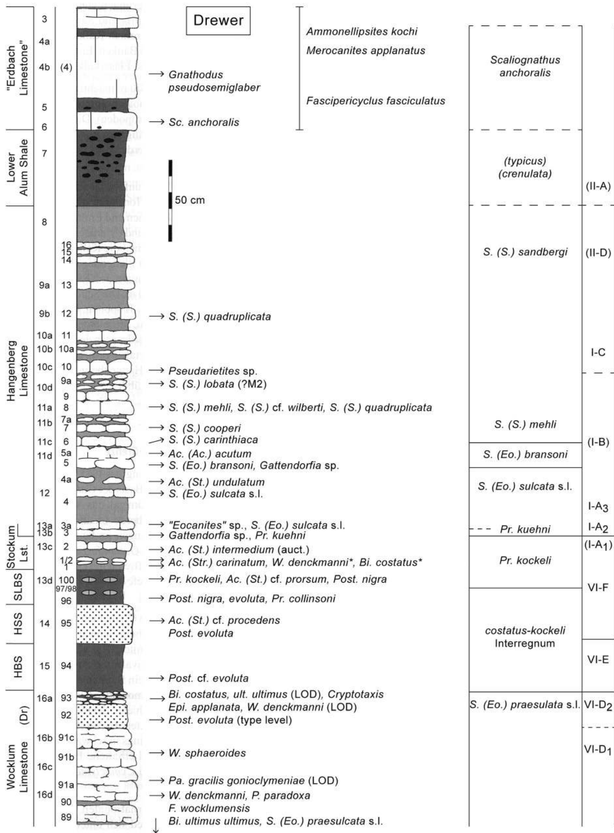
Fig. 14 Synthetic DCB succession of the Provincial Quarry Drewer near Beleecke, showing occurrences of index ammonoids and conodonts, originally re-drawn from Clausen and Korn (2008), here updated from
