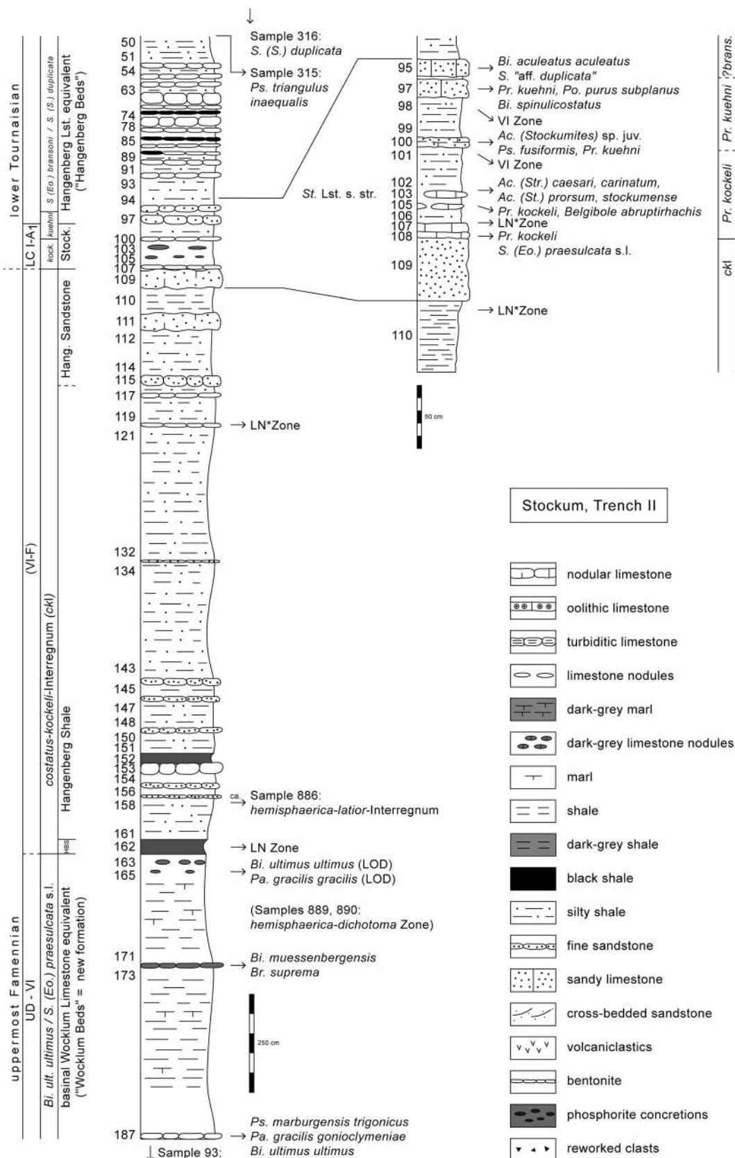
Fig. 13 Summary section log for the DCB transition at Stockum (re-drawn from the section log of Clausen et al. 1994, fig. 6) showing the occurrences of marker conodonts, ammonoids, and miospore zones. For
