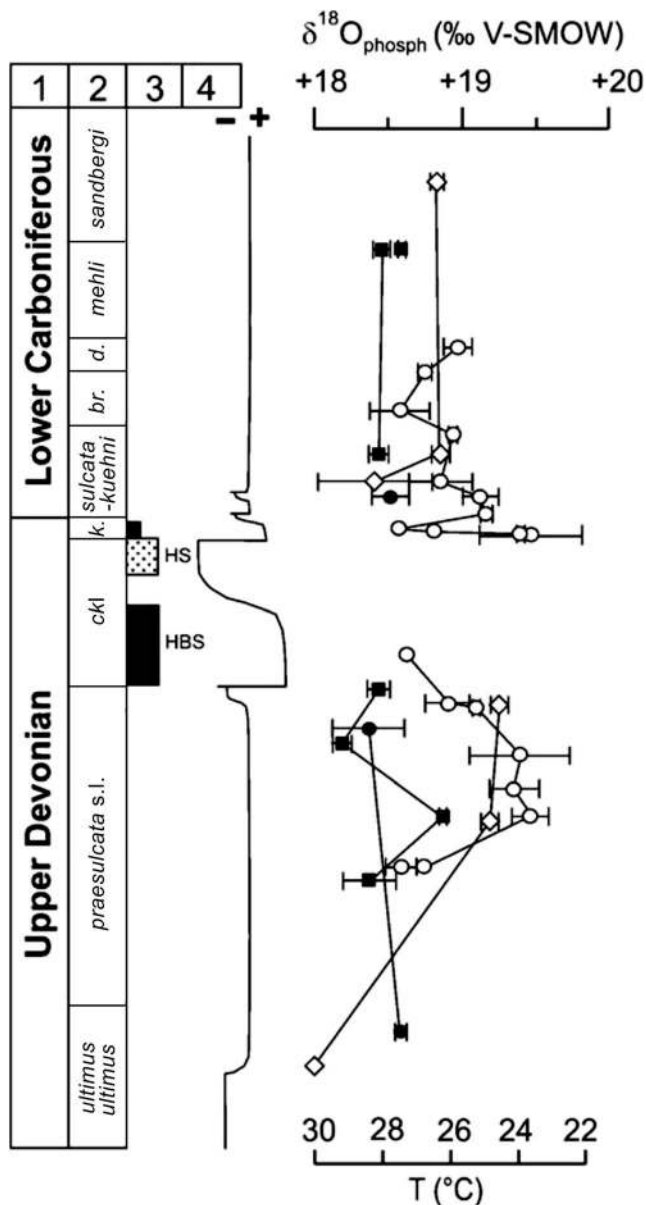
Fig. 5 Pelagic sea surface palaeotemperatures (black dots and squares) calculated from oxygen isotope values of conodont phosphate from the uppermost Famennian and basal Tournaisian of Hasselbachtal (dots) and the Oberrödinghausen Railway Cut (squares), extracted and modified from Kaiser et al. (2006, fig. 7). 1 chronostratigraphy, 2 conodont zonation (compare Fig. 1 to understand abbreviations), 3 marker units, 4 sea-level curve; HBS Hangenberg Black Shale, HS Hangenberg Shale/Sandstone.
