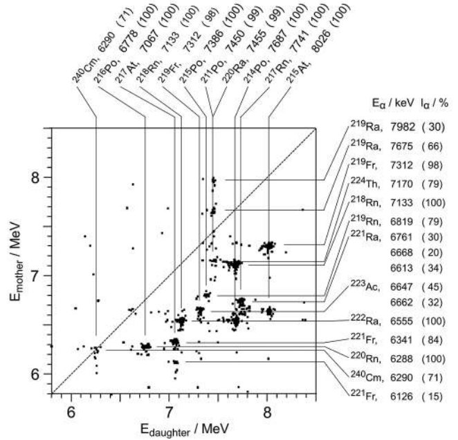
Fig. 6. Energies of mother-daughter delayed coincidences of events during the beam pauses within time and position windows of 1 s and \pm 1 mm, respectively. Given literature values of \alpha energies and intensities were taken from [64]. The spectrum includes data measured during 25 days beginning May 5. Strip numbers 5, 9, 13 and 15 are not included, see text for details.
