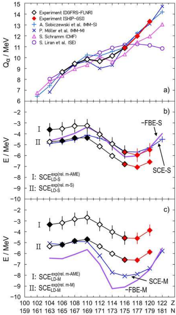
Fig. 10. Comparison of experimental and theoretical Q_\alpha values for nuclei of the \alpha -decay chain passing through the isotope ^{291}\text{Lv} (a). Experimental Q_\alpha values of nuclei from ^{271}\text{Sg} to ^{291}\text{Lv} were taken from [57]. Theoretical Q_\alpha values were taken from the macroscopic-microscopic models by Sobczewski et al. [54,55,117] (MM-S) and Möller et al. [97] (MM-M), the chiral mean-field model (CMF) by Schramm [36], and a semi-empirical model (SE) by Liran et al. [99]. Experimental shell-correction energies of the decay chain are compared with theoretical values of the MM-S model in (b) and of the MM-M model in (c). Experimental data with error bars are based on the AME mass of ^{267}\text{Rf} (filled symbol), from which the theoretical LD masses, LD-S and LD-M, were subtracted. Experimental data without error bars are based on the theoretical masses. They better reflect different trends between experiment and theory along the measured decay chains. In (b), (c) these masses were fitted to the theoretical masses of ^{271}\text{Sg} , ^{275}\text{Hs} and ^{279}\text{Ds} (filled symbols). Note that within an \alpha -decay chain the shape of the experimental SCE curves is fixed by the measured Q_\alpha values and the used theoretical LD masses. Curves without symbols show the negative values of the heights of the fission barriers, -FBE-S and -FBE-M , obtained in models MM-S and MM-M.
