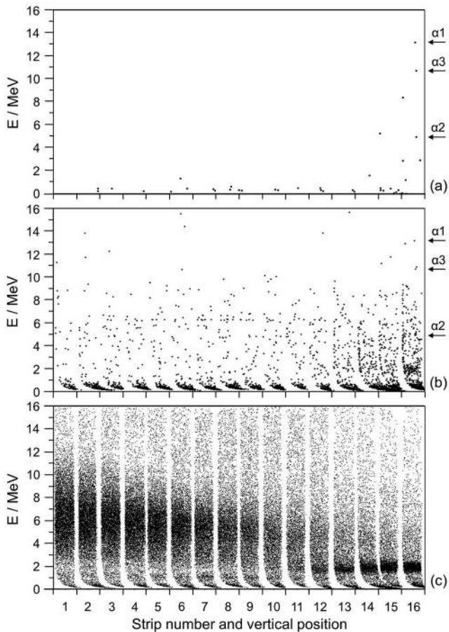
Fig. 8. Energy-position scatter plot of events measured with ((a), (b)) and without (c) the anti-coincidence condition with both TOF and veto detector signals. The measuring time was 5 s in (a) and 10 min in ((b), (c)) before and after the event \alpha_1 of the chain of the three signals from May 18, 2011. The spectra include events from both the 5.2 ms pulse and the 14.8 ms pause. The abscissa shows for each detector strip the vertical position ranging from 0 mm at the bottom to 35 mm at the top of the strip. For an explanation of the distribution of the background events see text. All three events of the chain are clearly seen on the upper half of detector strip 16 in (a), \alpha_1 and \alpha_3 also in (b) despite of the higher background. Note that \alpha_2 is an escape event for which only the energy loss in the stop detector is plotted. The event close to \alpha_3 in (b) has an energy of 10.857 MeV and a position of 26.0 mm. It occurred during the macro-pulse, 2.28 ms after its beginning and 393 s before \alpha_1 . This event is in reasonable agreement with the background rate of such signals determined in sect. 3.2.3. and is, therefore, excluded as a member of the decay chain. Visible in (b) at 6.3 MeV and distributed across strip numbers 3 to 13 are also decays of the background activities of ^{240}\text{Cm} and ^{220}\text{Rn} .
