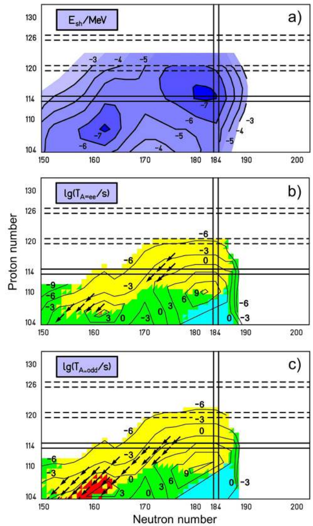
Fig. 1. Shell-correction energies in MeV taken from [16,18] (a) and dominating decay modes of even-even nuclei (b) and of even-odd nuclei (c). Using partial half-lives calculated in [16–18], the resulting dominating decay modes are plotted for \alpha decay (yellow), \beta^+ decay or electron capture (red), \beta^- decay (blue), and SF (green) for even-even nuclei in (b) and for even-odd nuclei in (c). Arrows mark measured decay chains starting at the even element isotopes ^{264}\text{Hs} , ^{270}\text{Ds} , ^{268}\text{Hs} , ^{270}\text{Hs} , ^{294}\text{118} , and ^{292}\text{Lv} in (b) and at ^{263}\text{Hs} , ^{269}\text{Ds} , ^{271}\text{Ds} , ^{277}\text{Cn} , ^{271}\text{Hs} , ^{285}\text{Fl} , ^{291}\text{Lv} , and ^{293}\text{Lv} in (c). The \alpha -decay chains end by SF in agreement with predictions.
