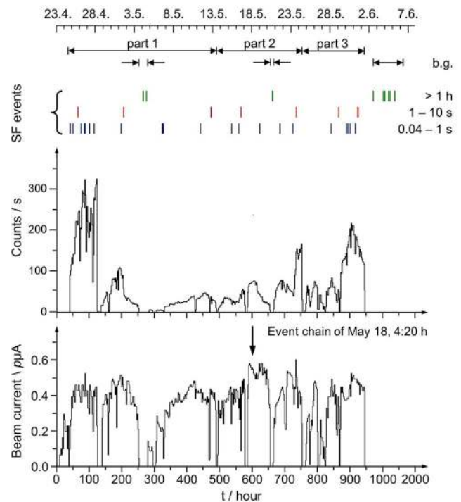
Fig. 4. Beam current (lower part, given is the average value in bins of 2 h) and rate of target like nuclei in the stop detector within an energy window from 18 to 40 MeV (middle part) plotted as a function of the beam time. See text for an explanation of the measured SF events shown on top of the figure. Two longer periods during and one after the irradiations were used for background measurements. These periods are shown in the row marked “b.g.” in the upper part of the figure. The time of the occurrence of the three events chain on May 18th is marked in the lower part.
