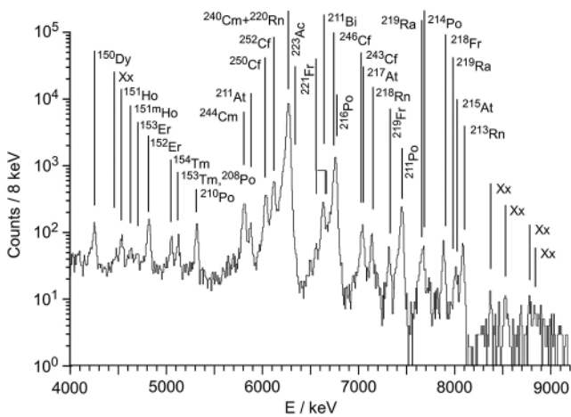
Fig. 5. Alpha singles spectrum taken during the beam-off periods. The spectrum shows all events occurring during the 14.8 ms pauses between the beam pulses and during the irradiation period of 25 days from May 5 to 30. Strip numbers 5, 9, 13 and 15 are not included, see text for details. The assignment of lines marked by “Xx” as element symbol is still uncertain. The energy scale is shifted by a mean value of 40 keV for compensating the fraction of the recoil energies contributing to the height of the detector signals. In that case the scale corresponds to the \alpha energies.
