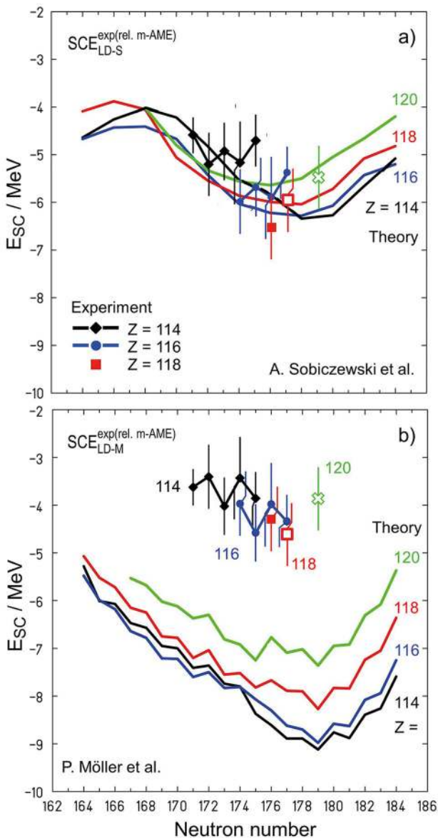
Fig. 11. Model-dependent experimental shell-correction energies of isotopes of elements flerovium, livermorium and 118 (filled symbols) and of the values deduced from the decays of nuclei tentatively assigned to ^{295}118 and ^{299}120 (open symbols, crosses for Z = 120 ) are compared with theoretical predictions of the MM-S model in (a) and of the MM-M model in (b). In (a) theoretical values of only the even-even nuclei are plotted. The difference between experimental data in (a) and (b) is due to differences of the LD masses of the two models MM-S and MM-M. The experimental SCE values with error bars are based on the mass estimates of the AME-2012 mass evaluation [90, 124]. The figure is a modified version of fig. 4 in [123].
