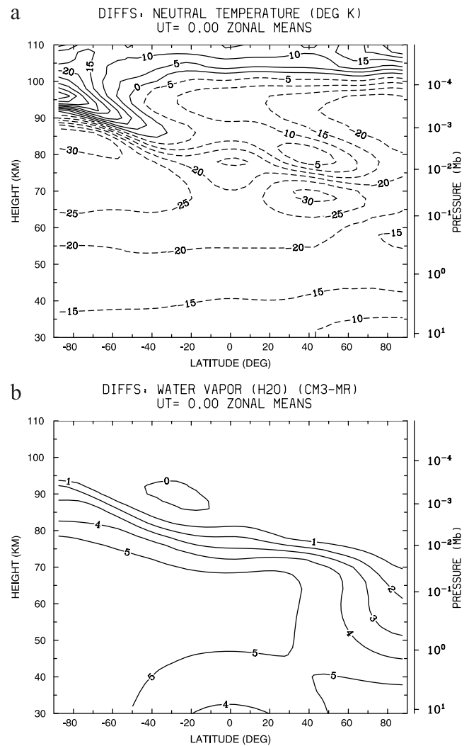
Figure 11. Calculated (a) neutral gas temperature and (b) H 2 O mixing ratio for the 2100 A.D. assumed scenario using the thermosphere-ionosphere-mesosphere electrodynamics general circulation model of the National Center for Atmospheric Research. The calculated difference fields for this case minus the present-day conditions are shown in Figure 11 for the above mentioned fields, respectively. Most calculations have assumed only a CO 2 -doubling scenario, but in this case, additional trace gas increases are considered, as shown in Table 6 (for detail see text).
