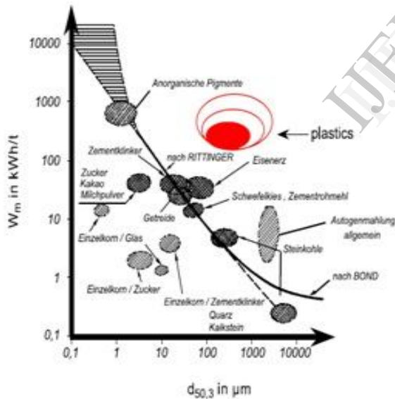
SPECIFIC WORK OF COMMINATION OF DIFFERENT MATERIALS DEPENDING ON THE PARTICLE SIZE (Rumpf, 1975)
