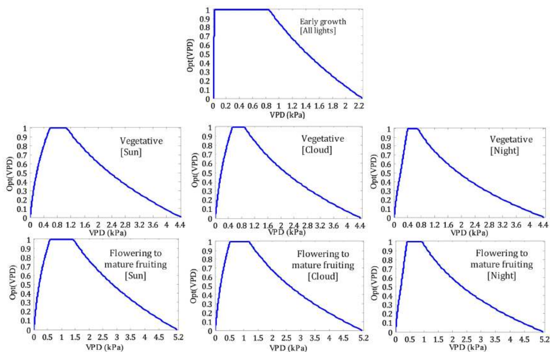
Fig. 3. Graphs of membership functions for defining optimality degrees of vapour pressure deficit at different light condition and growth stages for the ‘Caruso’ greenhouse tomato cultivar, adapted from (Shamshiri et al. , 2017b).
