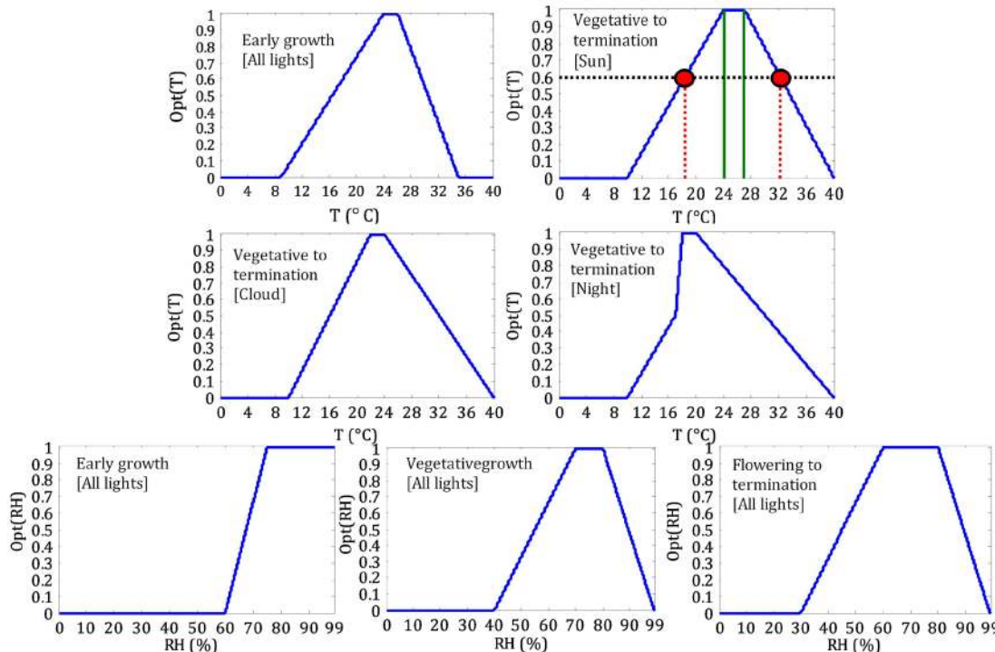
Fig. 2. Graphs of growth response function for defining optimal air temperature and relative humidity for the ‘Caruso’ greenhouse tomato cultivar at different growth stages and light conditions, adapted from (El-Attal, 1995).
