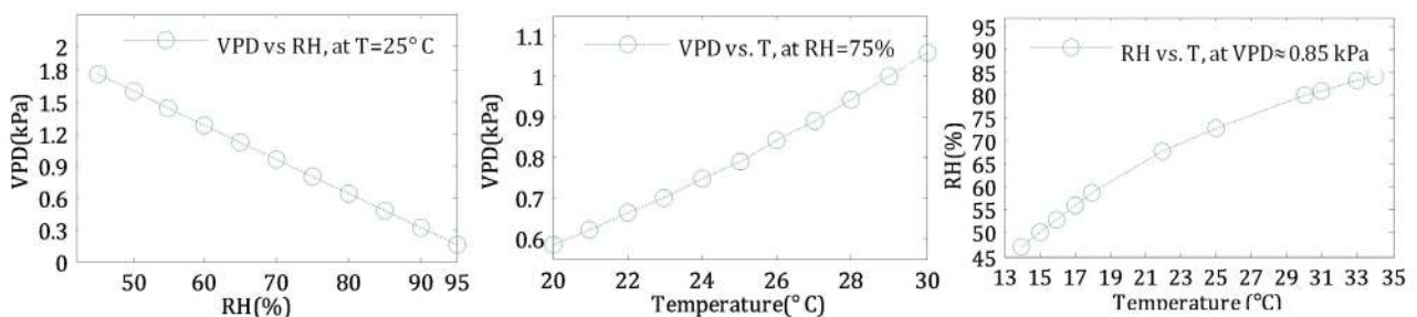
Fig. 4. Demonstration of VPD in relation to variable and constant T and RH .
