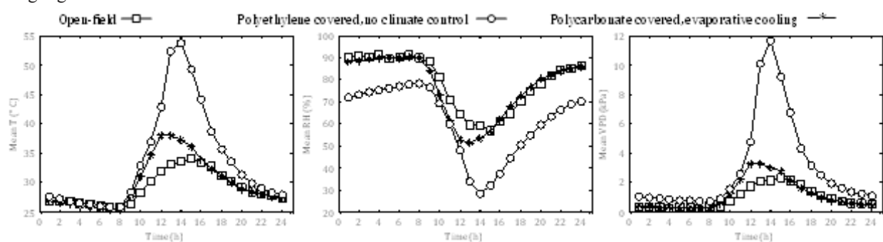
Fig. 5. Effects of greenhouse cladding and cooling systems on day and night T , RH and VPD under tropical climate conditions (Shamshiri et al. , 2016b).
