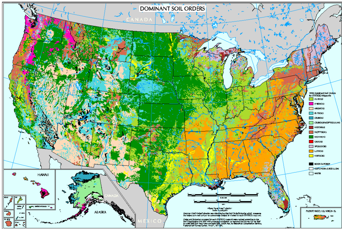
Figure 8. Soils map of the United States. (From http://www.nrcs.usda.gov/technical/land/lgif/m40251.gif .)
