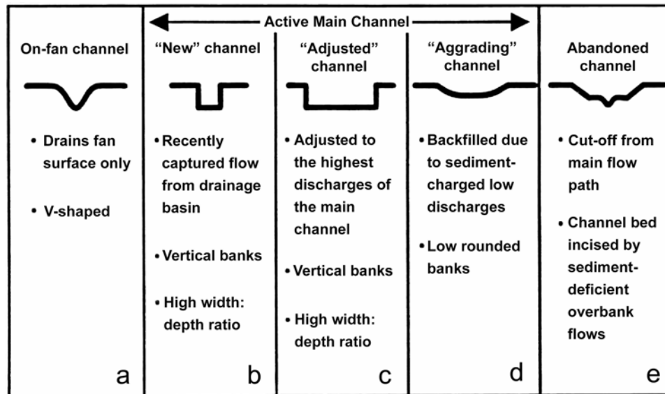
Figure 19. Five channel morphologies observed on alluvial fans in southern Arizona. Note that a single channel reach can go through each phase of channel development through time, and each stage of development can be observed at different places on a fan at the same time. (Modified from Field 2001.)
