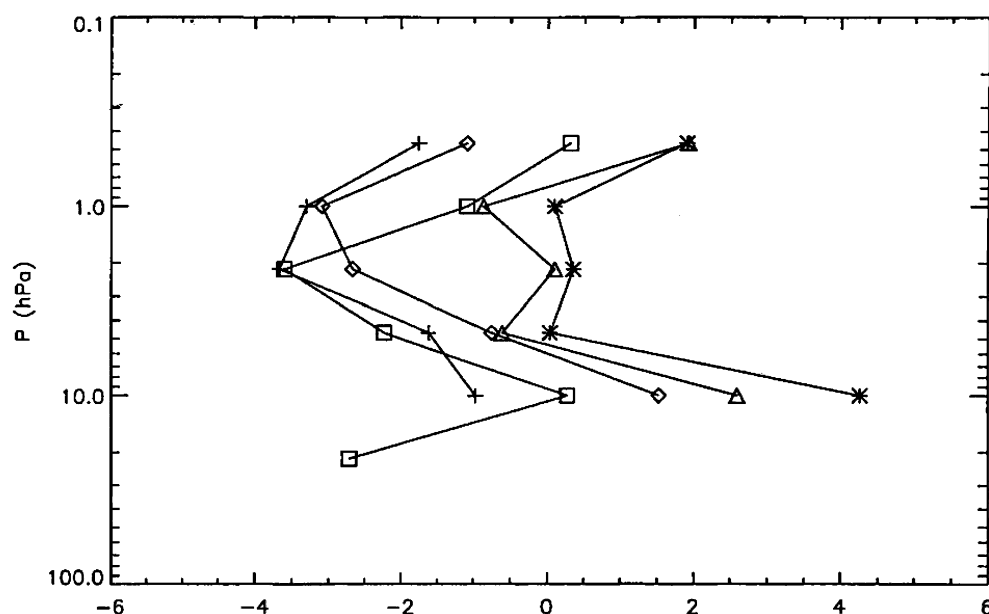
Fig. 4 Average differences between the closest MLS profile and the JPL lidar at TMF (pluses); the CNRS lidar at OHP (asterisks); the GSFC lidar at TMF (triangles), and at OHP (squares) from Fishbein et al. 54 (Copyright 1996, Journal of Geophysical Research ).
