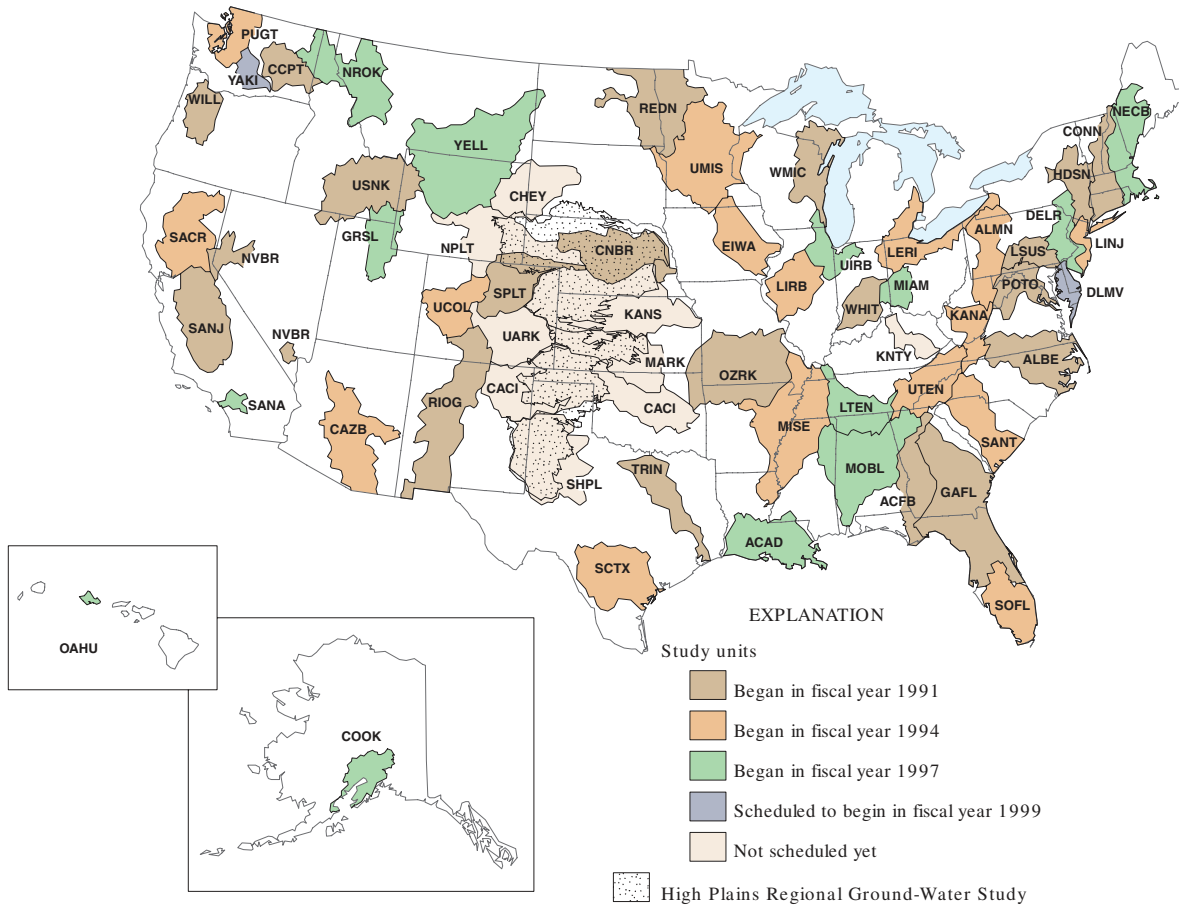
Figure 7. Location of National Water-Quality Assessment Program study units.
