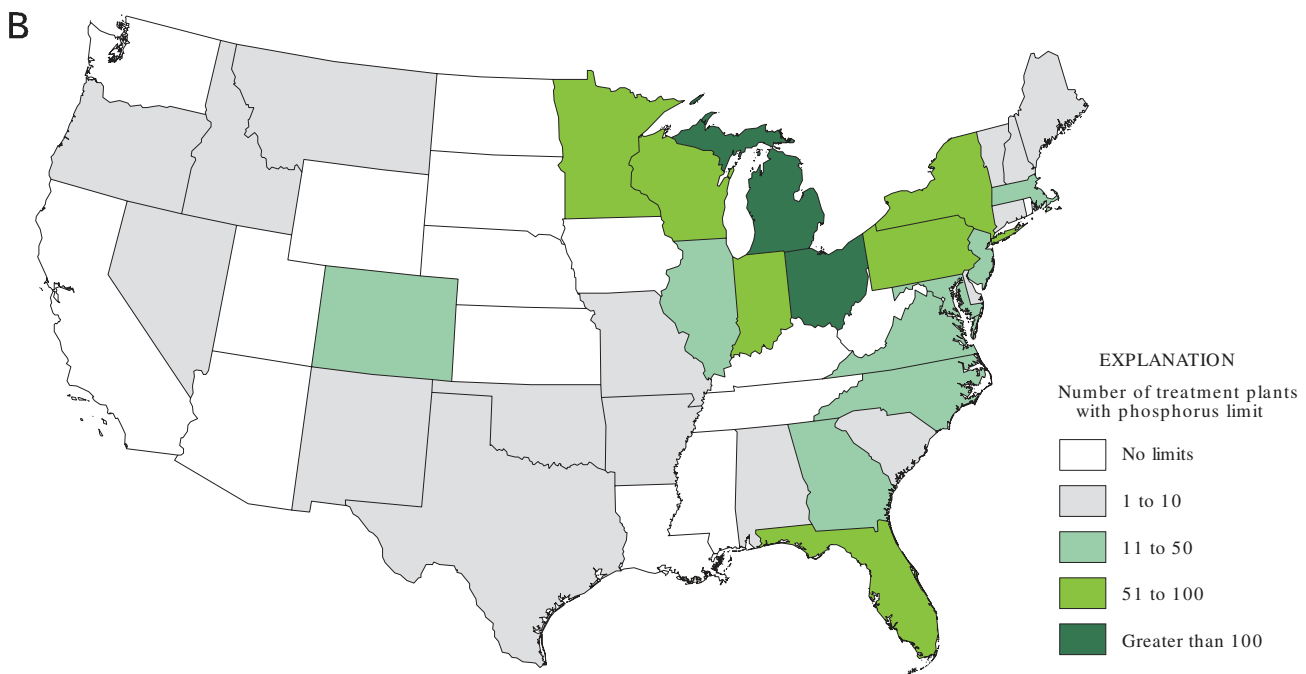
Figure 3. (A) States with phosphate detergent bans, and (B) number of wastewater-treatment plants with phosphorus limits. Alaska and Hawaii have neither bans nor phosphorus limits.
