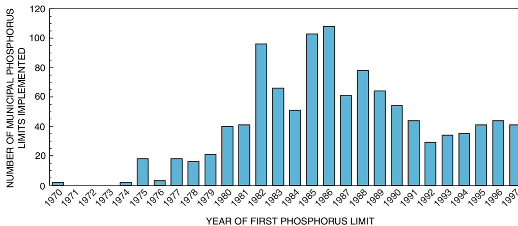
Figure 5. Implementation of phosphorus effluent limits by year, 1970-1997 [source of data: U.S. Environmental Protection Agency Permit Compliance System data-base retrieval, 1997].
