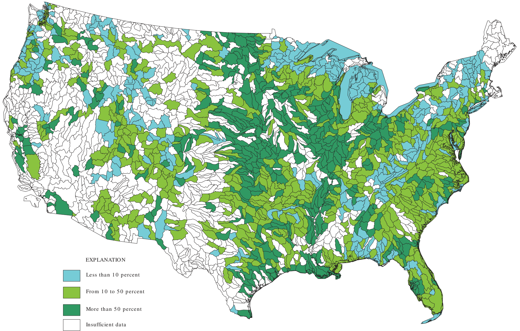
Figure 6. Percentage of total phosphorus concentrations that exceeded recommended limit of 0.1 milligram per liter, by hydrologic unit, 1990-95 [source of data: U.S. Environmental Protection Agency STORET data base].
