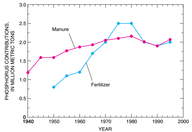
Figure 1. Contributions to the environment of phosphorus from fertilizer and manure, 1940-95 [source of data: fertilizer use from Puckett (1995); manure use estimated using method of Alexander and Smith (1990), and animal counts from U.S. Bureau of the Census (1976, 1995)].
