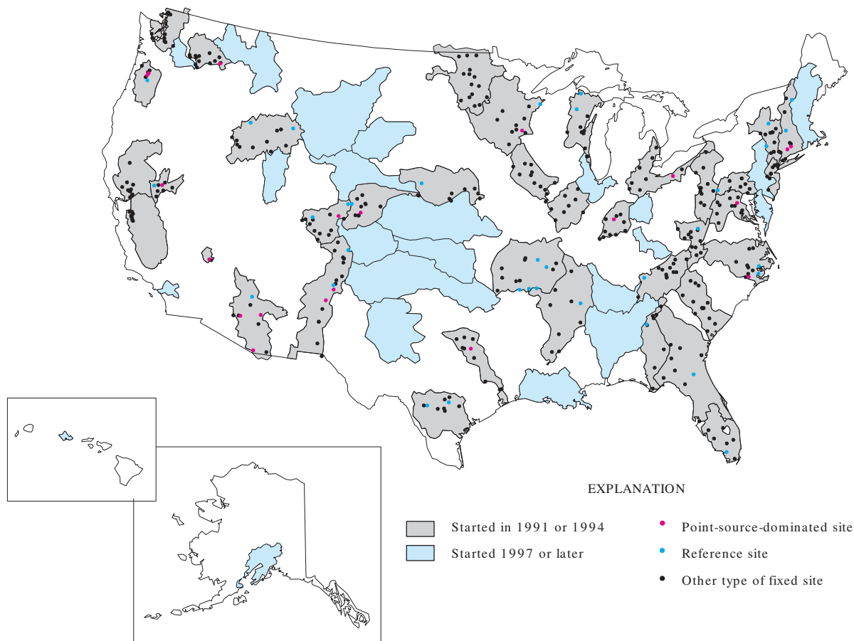
Figure 9. Location of National Water-Quality Assessment Program fixed monitoring sites.
