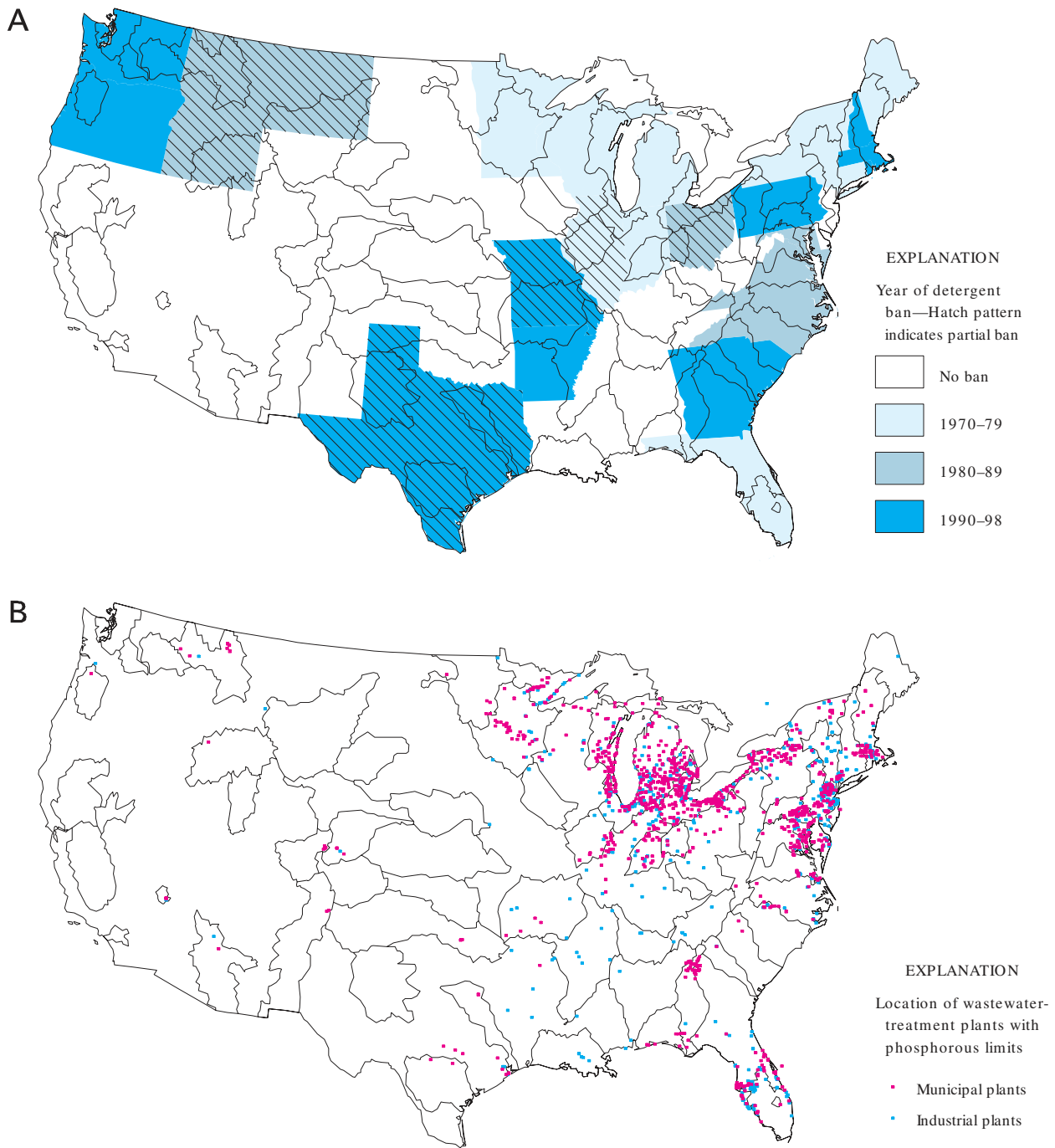
Figure 8. Location of National Water-Quality Assessment Program study units, (A) States with phosphate detergent bans, and (B) locations of industrial and municipal wastewater-treatment plants having phosphorus limits.
