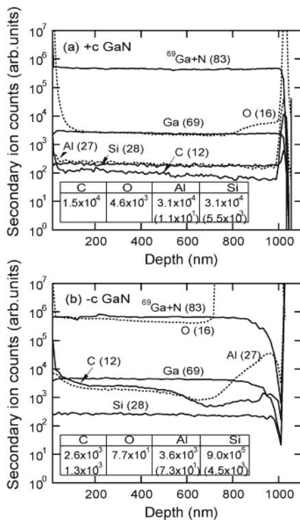
Figure 22. Depth profiles of C - , O - , Al - , Si - , Ga - and GaN - for (a) +c GaN and (b) -c GaN films of 1µm in thickness. The intensities of impurities normalized to the GaN - count are listed at the bottom of each figure. The values normalized to the Ga+Ga + ion in the brackets are evaluated from depth profiles using and O 2 + primary beam [after Ref. 135]. The Al, C and O impurities were more readily incorporated into -c GaN films.
