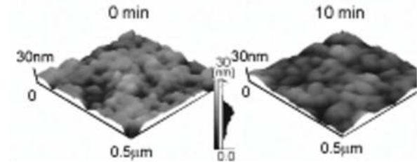
Figure 16. AFM images of annealed buffer layers on nitrided sapphire substrates before (on the left) and after (on the right) dipping in KOH solution for each time stated. (a) The sample deposited under a V/III ration of 20 000 and annealed in the H 2 and N 2 mixed ambient for 20min, and (b) the sample deposited under a V/III ratio of 5000 and annealed in an N 2 ambient for 20min. [after Ref. 117]
