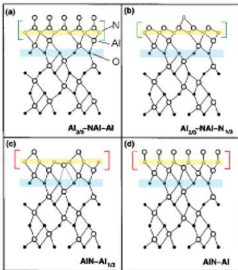
Figure 9. Models for the AlN thin films on c -plane sapphire substrates given in Ref. [58]. The color regions are added to explain the theoretical predictions. The structures in the brackets correspond to the polar structures of AlN described in Ref. [84]. (a) and (b) correspond to a +c polar surface. (c) and (d) to -c polarity.
