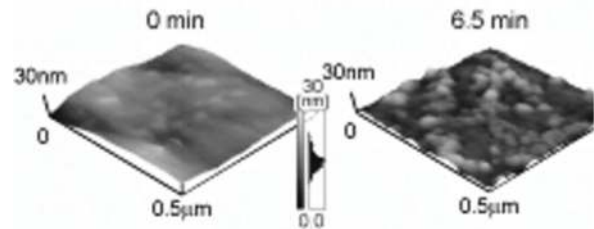
(b) V/III 2000 on nitrided sapphire
