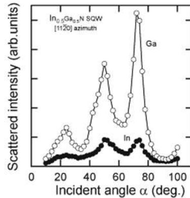
Figure 7. Incident angle dependence of Ga and In scattered intensity at the [11\bar{2}0] azimuth for \text{In}_{0.5}\text{Ga}_{0.5}\text{N} SQW. Variation of both the Ga and In signals indicates +c polarity judging from the CAICISS results on ZnO bulk given in Fig. 5. Indium atoms incorporated into an \text{In}_x\text{Ga}_{1-x} SQW were found to occupy substitutional Ga sites. [52]]
