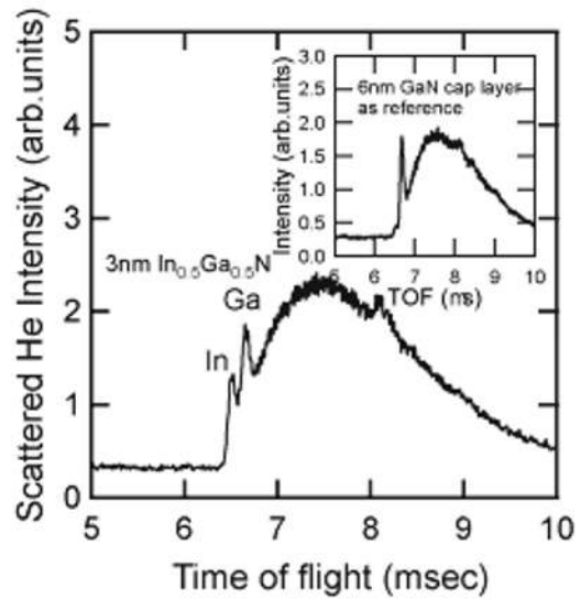
Figure 6. TOF spectrum of the backscattered \text{He}^+ ions used in the CAICISS analysis of an \text{In}_{0.5}\text{Ga}_{0.5} SQW when the ion beam was irradiated at normal incidence to the sample. The inset depicts the TOF spectrum for \text{In}_{0.2}\text{Ga}_{0.8} capped with 6-nm-thick GaN as a reference [after Ref. 51]. The In and Ga signals can be detected separately for each time-of-flight. The inset indicates how CAICISS analysis detects a region several nm deep below the surface.
