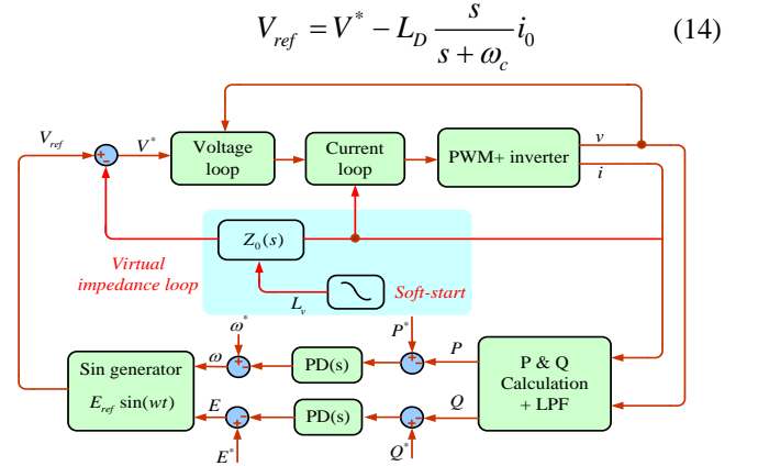
Fig. 9. The control scheme of droop control with virtual output impedance.
