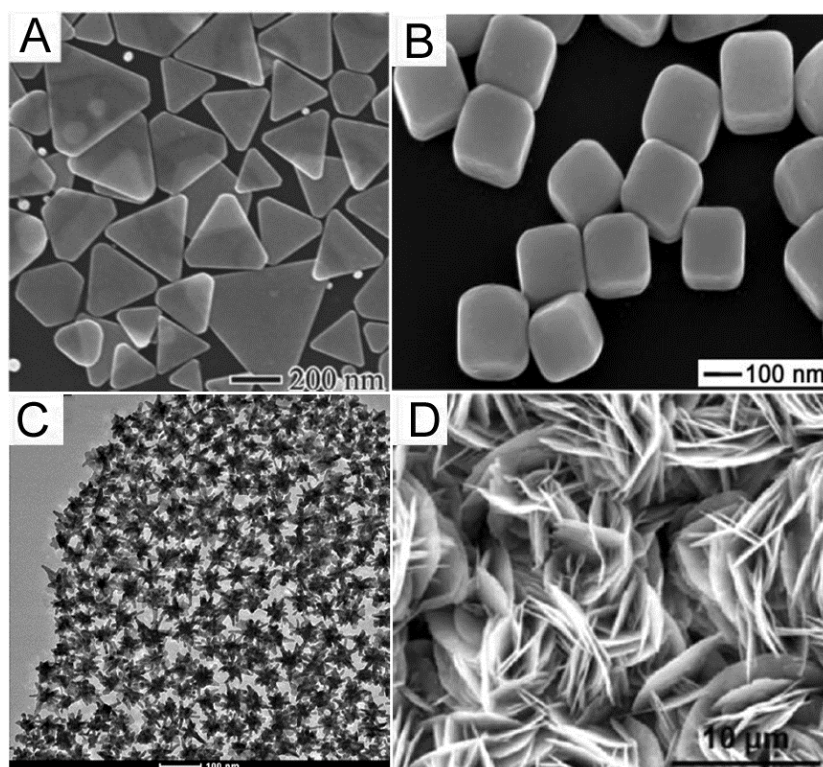
Figure 4. Representative metallic nanomaterials with different geometric morphologies: (A) SEM images of Ag nanoprisms [89] (reproduced with permission from Yang et al. , published by John Wiley and Sons, 2014); (B) SEM images of Ag nanocubes [90] (reproduced with permission from Sun et al. , published by AAAS, 2002); (C) TEM images of Au nanostars [94] (reproduced with permission from Yuan et al. , published by ACS, 2012); (D) SEM images of Ag nanosheets [96] (reproduced with permission from Yan et al. , published by ACS, 2012).
