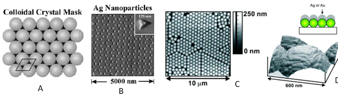
Figure 5. Schematic illustration of a colloidal crystal mask (A) and representative AFM image (B) of Ag nano-triangular structures. Ambient contact mode atomic force microscope image of 200-nm Ag over 542-nm diameter polystyrene spheres: (C) array of spheres ( 10\ \mu\text{m} \times 10\ \mu\text{m} ) and (D) image ( 600\ \text{nm} \times 600\ \text{nm} ) of one sphere showing substructure roughness with schematic illustration [97,101]. (Reproduced with permission from Van Dyne et al. , published by ACS 2001, 2002.)
