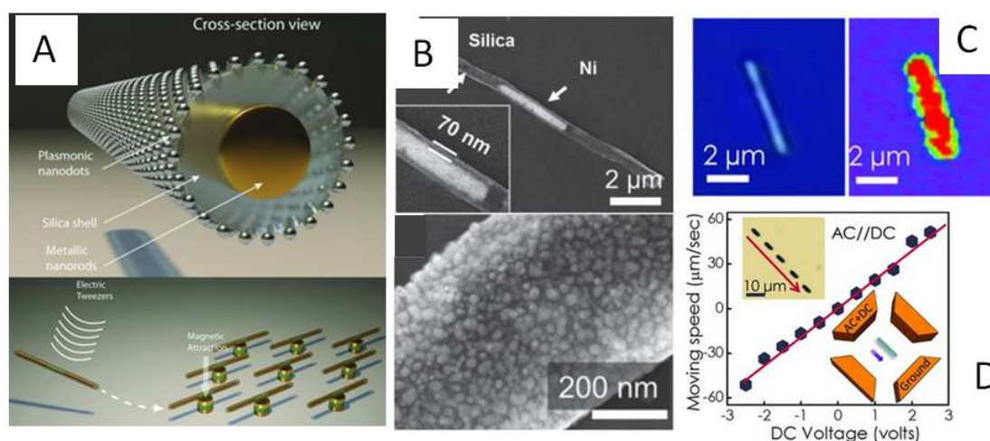
Figure 7. (A) (Top) Structure of a tri-layer nanocapsule; (bottom) with the electric tweezers, nanocapsules can be transported and assembled onto a pre-patterned array of nanomagnets by utilizing the magnetic attraction force between the Ni segments in the nanocapsules and the magnetic layers inside the nanomagnets [108] (reproduced with permission from Xu et al. , published by John Wiley and Sons, 2012); (B) SEM images of silica nanotubes embedded with Ni nanomagnets and a close view of the AgNPs on the nanotube surface [109] (reproduced with permission from Xu et al. , published by John Wiley and Sons, 2013); (C) Raman mapping profile of 1 \mu\text{M} Rhodamine 6G dispersed on a tri-layer nanocapsule shows uniform SERS intensity on the entire surface of the nanocapsules. ( 1655 \text{ cm}^{-1} , scan step 250 nm, integration time 0.5 s) [109] (reproduced with permission from Xu et al. , published by John Wiley and Sons, 2013); (D) Electric tweezers using AC and DC configurations on quadruple electrodes for the manipulation of nanocapsules [108] (reproduced with permission from Xu et al. , published by John Wiley and Sons, 2012).
