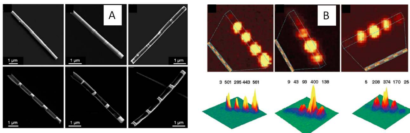
Figure 6. (A) SEM images of on-wire lithography (OWL)-generated nanodisk arrays with various geometries; (B) Confocal Raman microscopy images of gapped nanowire structures functionalized with methylene blue (MB) [104]. (Reproduced with permission from Qin et al. , published by National Academy of Sciences, USA, 2006.)
