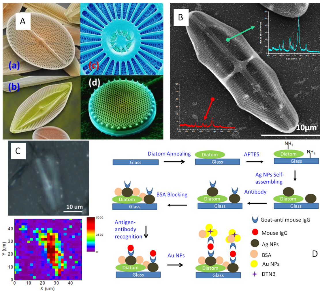
Figure 10. (A) SEM images of various diatom species with different frustules [141] (reproduced with permission). (B) SEM image of the hybrid diatom-plasmonic SERS substrates [151] (reproduced with permission from Yang et al. , published by John Wiley and Sons, 2014). (C) The 1 μM R6G Raman mapping results from the hybrid diatom-plasmonic SERS substrate [150] (reproduced with permission from Ren et al. , published by IEEE, 2014). (D) Schematic diagram of the diatom-plasmonic SERS immunoassay using a standard antigen-antibody model.
