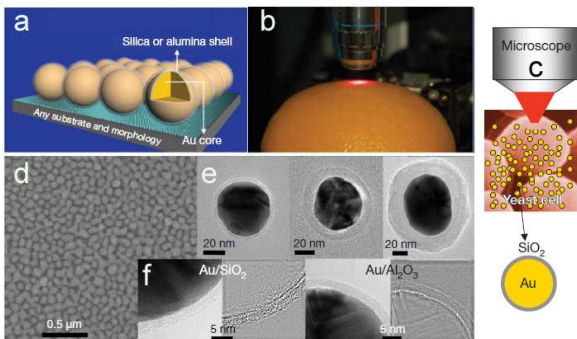
Figure 2. (a) The working principles of the shell-isolated nanoparticle-enhanced Raman spectroscopy (SHINERS) mode; (b) in situ inspection of pesticide residues on fruit by SHINERS; (c) in situ probing of biological structures by SHINERS; (d) SEM image of a monolayer of Au/SiO 2 nanoparticles on a smooth Au surface; (e) HRTEM images of Au/SiO 2 core-shell nanoparticles with different shell thicknesses; (f) HRTEM images of Au/SiO 2 nanoparticle and Au/Al 2 O 3 nanoparticle with a continuous and completely packed shell about 2 nm thick [67]. (Reproduced with permission from Li et al. , published by Nature Publishing Group, 2010.)
