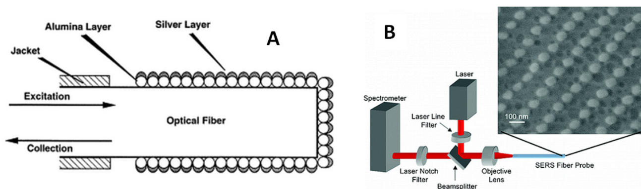
Figure 11. (A) Fiber-optic SERS sensors through the incorporation of alumina nanoparticles and silver coatings onto the single mode fiber probe tip [154] (reproduced with permission from Stokes et al. , published by Elsevier, 2000). (B) Schematic depiction of the configuration used to characterize the SERS fiber optic probe and a scanning electron micrograph of an array of gold optical antennas on the facet of a fiber [155]. (Reproduced with permission from Smythe et al. , published by ACS, 2009).
