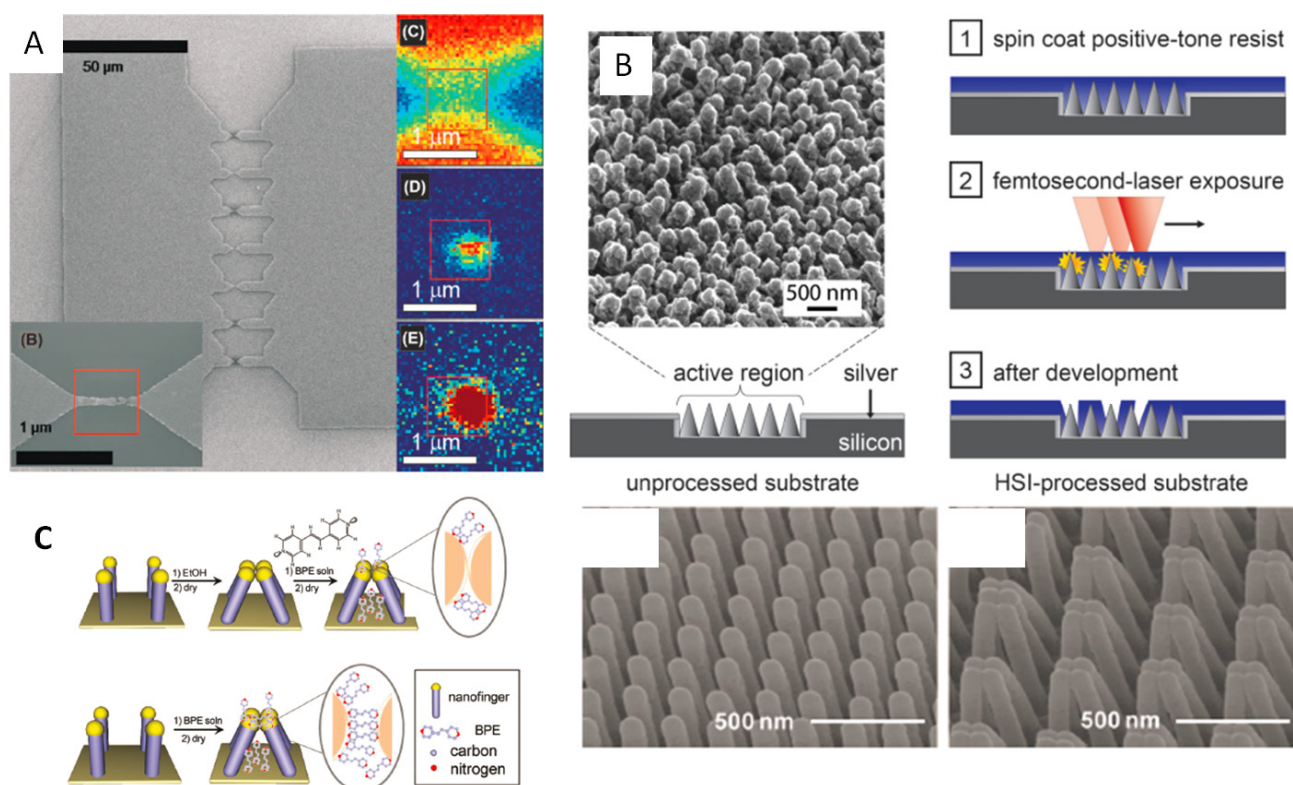
Figure 8. (A) Electro-migrated gaps from [122] (reproduced with permission from Ward et al. , published by ACS, 2007). (B) Helium ion microscope image ( 45^\circ ) and schematic diagram of multiphoton-lithography SERS substrate (left). Hot-spot isolation (HSI) process (right): (1) diluted positive-tone photoresist is spin-coated onto a SERS substrate to cover the surface; (2) a femtosecond laser pulse train is scanned over the surface, selectively exposing the photoresist covering electromagnetic hot-spots; (3) the photoresist is developed, and the SERS hot-spots are uncovered [123] (reproduced with permission from
