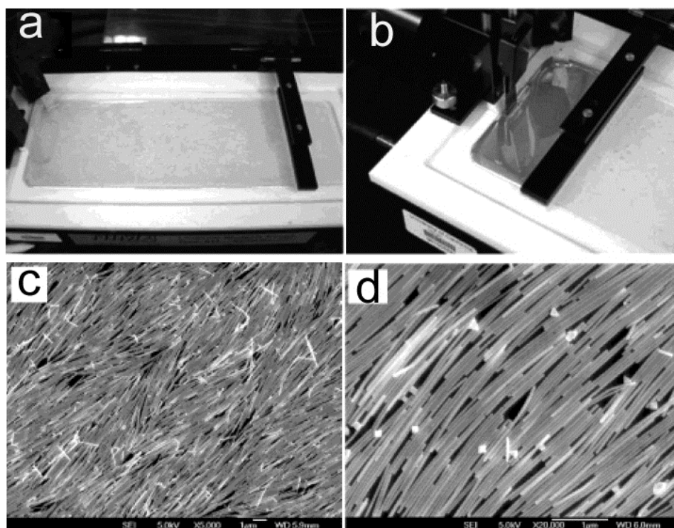
Figure 3. Photographs of Langmuir–Blodgett (LB) nanowire assembly process ( a,b ) at different compression stages. SEM images ( c,d ) of the Ag nanowire monolayer deposited on a silicon wafer at different magnifications [75]. (Reproduced with permission from Tao et al. , published by ACS, 2003.)
