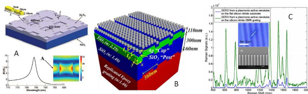
Figure 9. (A) (Top) The geometry of the dielectric grating structure with silver nanorod optical antennas on 2D silicon nitride grating surface. (Bottom right) Field map |E|/|E_0| at the surface of the grating at resonance. (Bottom left) |E|/|E_0| versus wavelength calculated by rigorous coupled wave analysis (RCWA) at Point A as marked by the inset to the right. |E_0| is the magnitude of the incident electric field [138] (reproduced with permission from Li et al. , published by American Institute of Physics, 2009). (B) Schematic diagram of PC-SERS substrate of SiO 2 -Ag “post-cap” nanostructure with a thickness of the SiO 2 layer of 75 nm and a thickness of the Ag layer of 20 nm by the oblique angle deposition method [139] (reproduced with permission from Kim et al. , published by Optical Society of America, 2010). (C) Measured 1 \mu M R6G Raman spectrum from the plasmonic nanotube on the flat Si 3 N 4 substrate and from the plasmonic nanotube on the GMR grating. The inset figures show the SEM image of the grating and the optical image of the plasmonic nanotube on top of the grating [41] (reproduced with permission from Xu et al. , published by American Institute of Physics, 2012).
