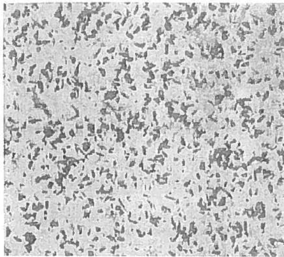
Fig.6. The microstructure of gas injected 17vol.%SiC/Mg composite [Ref. 92].
