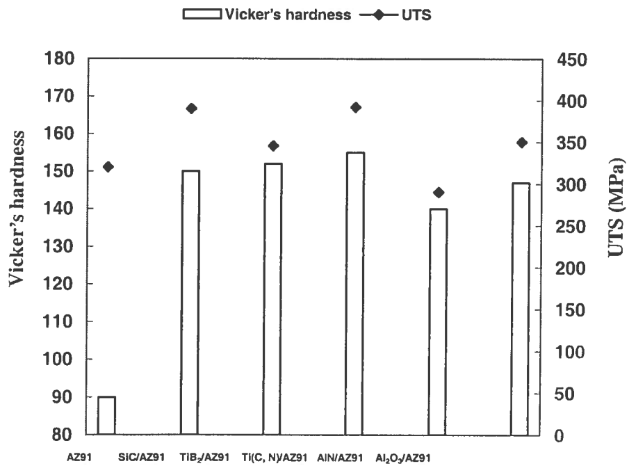
Fig. 11. Strength and hardness of AZ91 reinforced with different particles [Ref. 152].
