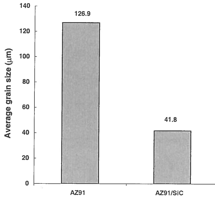
Fig. 9. The grain size of AZ91 and SiC/AZ91 composite [Ref. 126].
