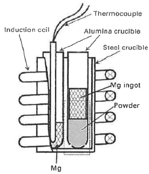
Fig. 4. The setup of Mg infiltration in mixed SiC and SiO 2 powders [Ref. 89].
