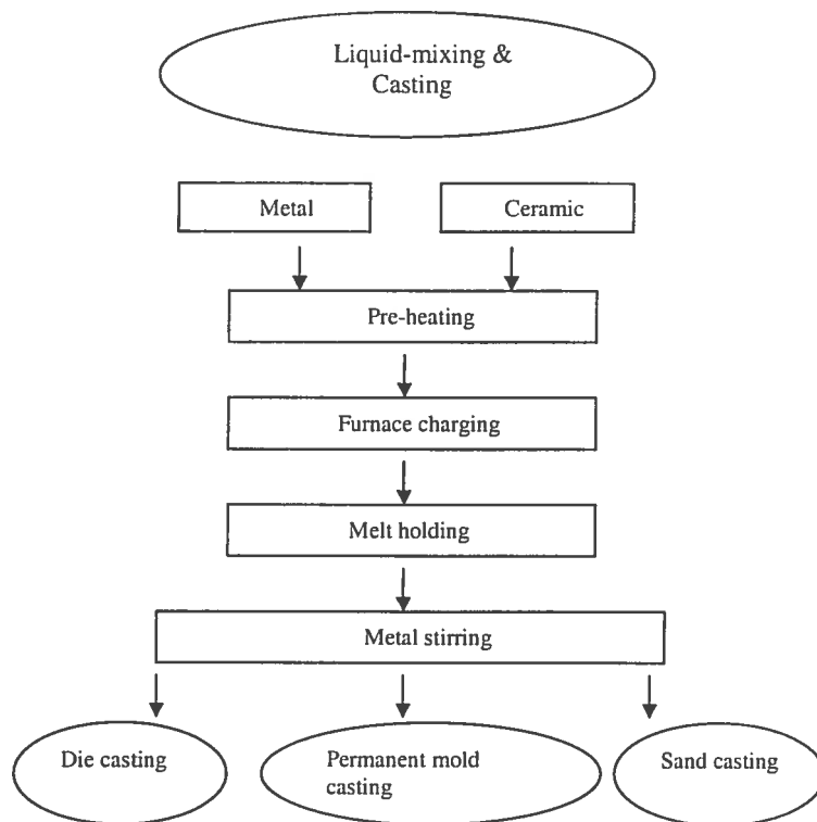
Fig. 1. The process of stir casting [Ref. 19].
