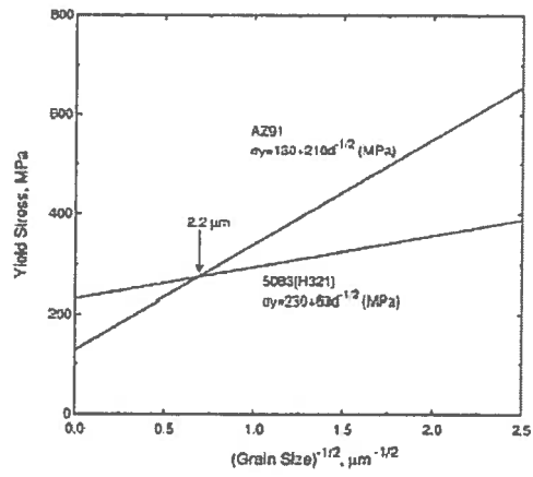
Fig. 8 . The yield strength and grain size of AZ91 and 5083 alloys [Ref. 125].
