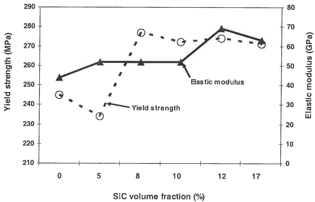
Fig. 7. Yield strength and elastic modulus of injected SiC/AZ91 composite [Ref. 92].
