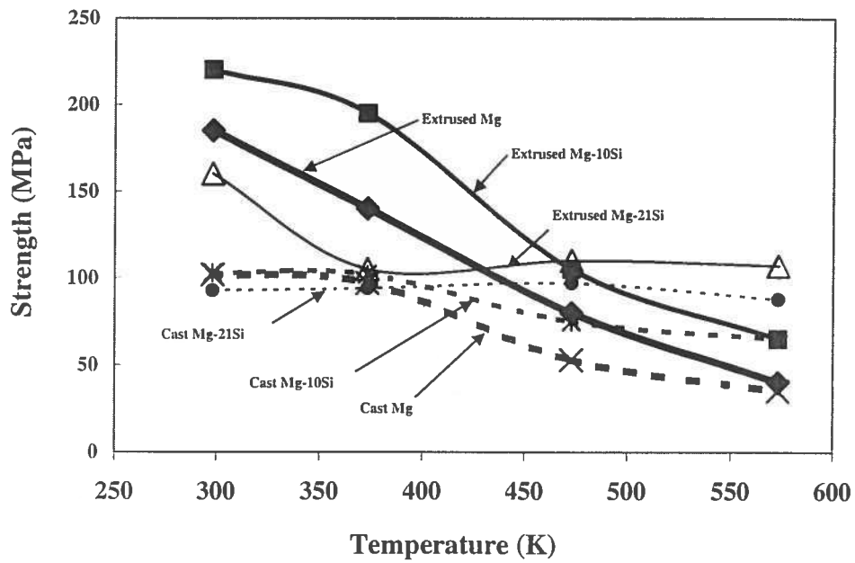
Fig. 3. The tensile strength of extruded and cast Mg-Si alloys [Ref. 60].
