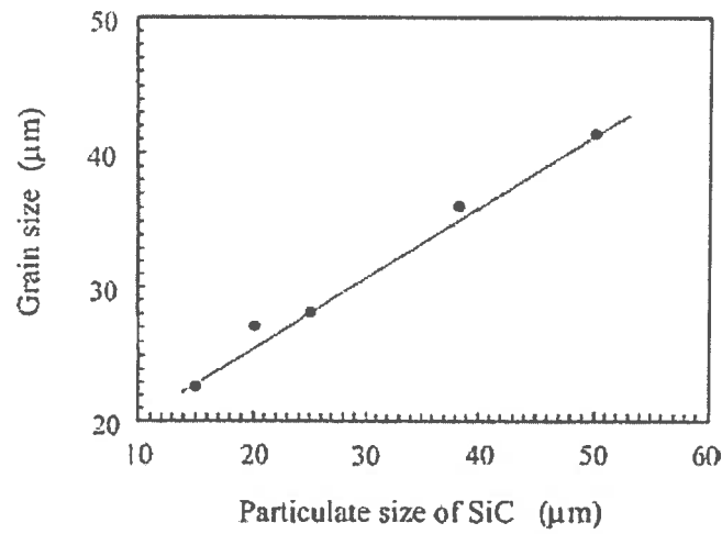
Fig. 10. SiC particle size and magnesium composite matrix grain size [Ref. 128].
