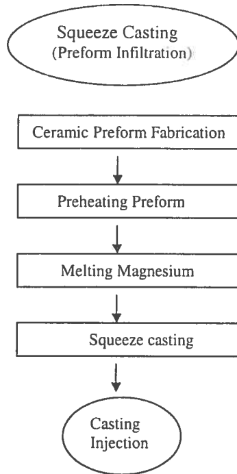
Fig. 2. The process of squeeze casting [Ref. 2].
