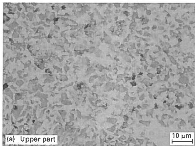
Fig. 5. The microstructure of the infiltrated SiC/Mg composite [Ref. 89].
