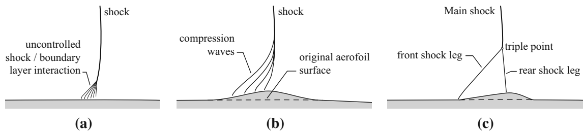
Fig. 2 Effect of SCBs on shock structure: a no-control case; b compression waves produced by a smooth contoured bump [4]; c λ-shock foot structure produced by a wedge bump (reproduced from [26] with permission of Hideaki Ogawa)
