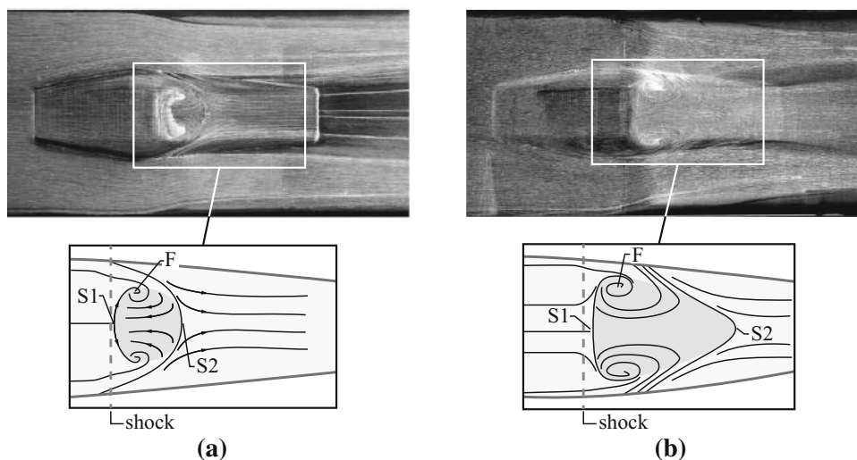
Fig. 16 Effect of streamwise pressure gradient on shock-induced separation topology: a flat plate, from [7]; b data from the set-up of [8]
