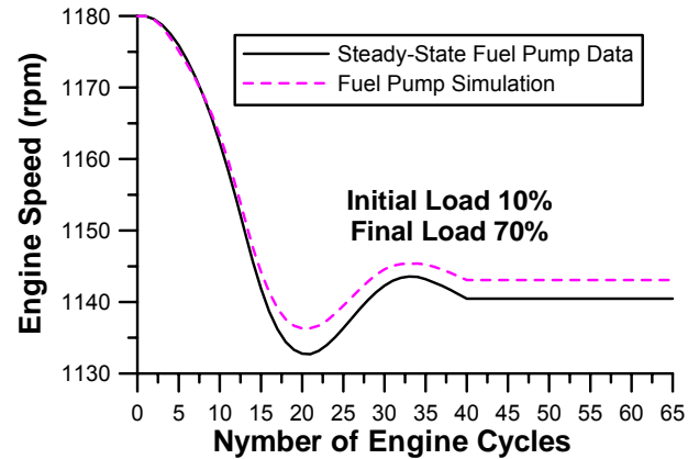
Figure 5b. Effect of fuel pump modeling on the predictions of transient engine operation
