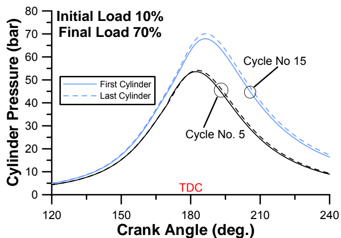
Figure 8. Effect of multi-cylinder modeling on the predictions of transient engine operation
