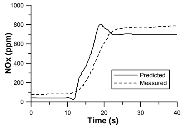
Figure 7a. Comparison between predicted and measured NOx emissions under engine load acceptance (adapted from [98])
