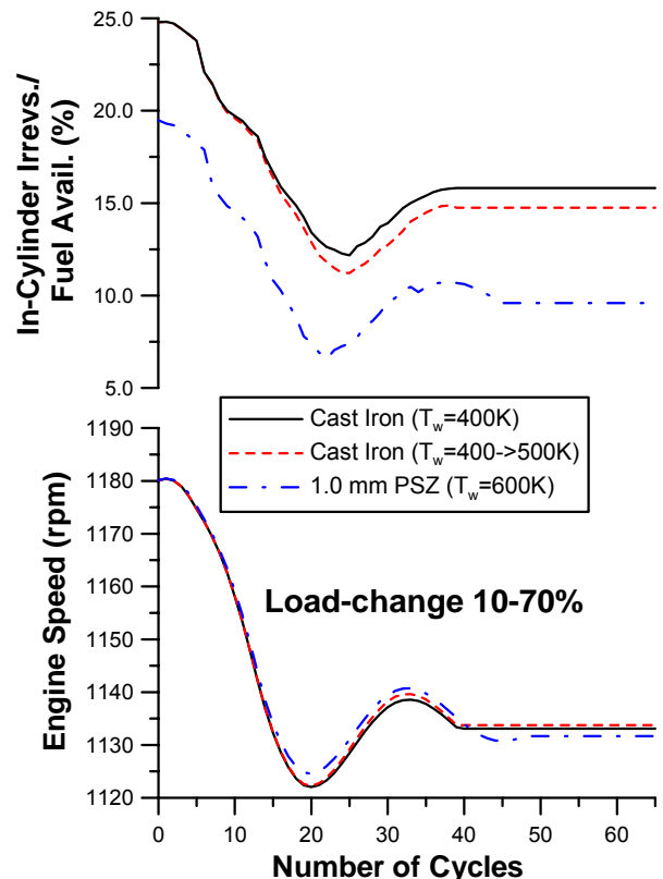
Figure 19. Effect of cylinder wall insulation on the second-law diesel engine transient performance after a ramp increase in load
