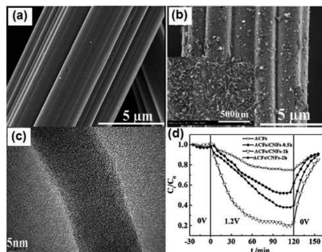
Fig. 13 SEM images of (a) ACFs and (b) ACFs/CNFs-1 h; (c) TEM image of ACFs/CNFs-1 h; (d) electrochemical process for the different electrodes in NaCl solution. Initial 30 min: physical adsorption; subsequent 120 min: electrosorption; final 30 min: desorption. The inset in (b) is the corresponding magnified image. (Reproduced with permission from ref. 102.)
