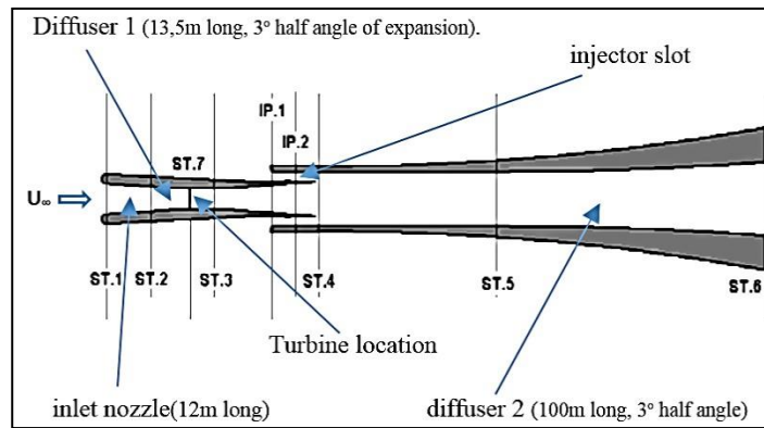
Fig. 17 The ejector assisted diffuser geometry [76].
