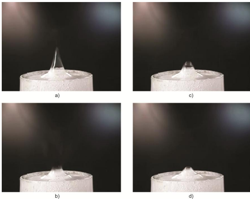
Figure 2. Rupture process of a bubble under an electrostatic field; (a) the thinning polymer bubble, (b) the bubble is broken somewhere on the top half, the small segments are ejected upwards to the receiver, (c) and (d) the bottom half retracts to form a daughter bubble
