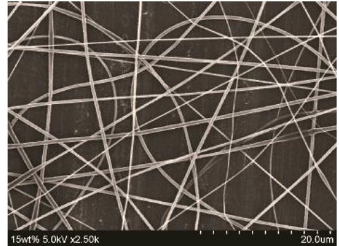
Figure 4. Continuous nanofibers ranging from 89 nm to 1,012 nm. A 15 wt.% PLA/DMF solution with molecular weight M_w \approx 100000 is used. The applied voltage is 15 kV and the received distance is 15 cm
