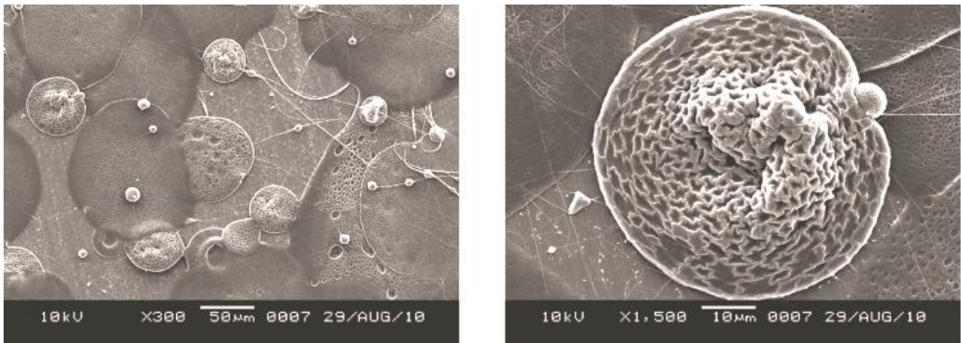
Figure 16. SEM images of the porous PBST electrospun mat with the voltage supplied 30 kV
