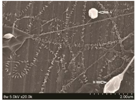
Figure 7. Discontinuous backbone-like wrinkled materials. The spinning condition is same with that for fig. 3. The average width is 154.33 nm, the average pitch is 141.4 nm. A is an irregular particle, B is a spindle-like structure
