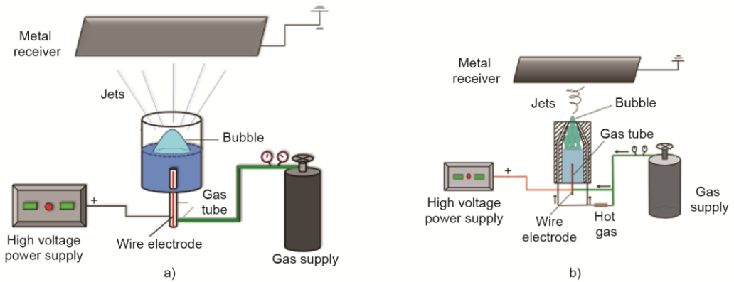
Figure 1. The experimental set-up of the bubble electrospinning; (a) bubble electrospinning, (b) blown bubble spinning
