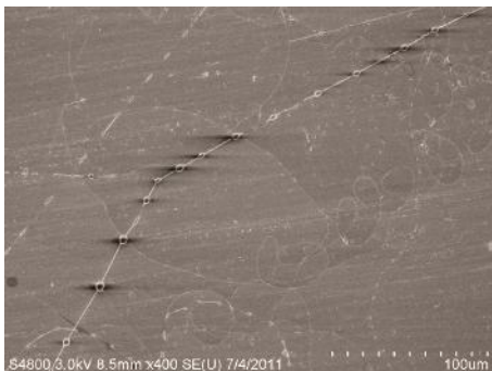
Figure 11. Beads in electrospun fibers by bubble electrospinning
