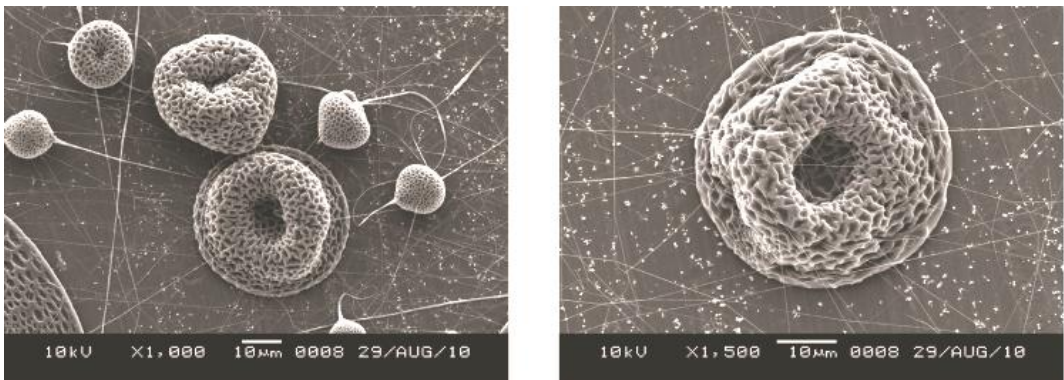
Figure 17. SEM images of the porous PBST electrospun mat with the voltage supplied 33 kV
