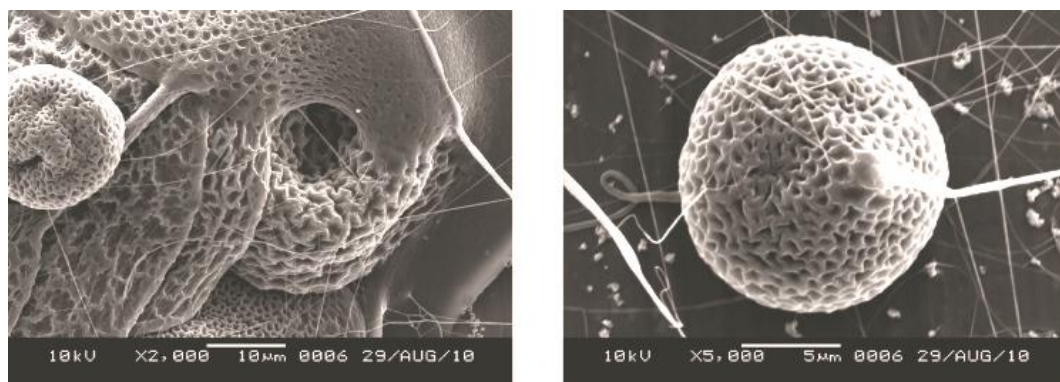
Figure 15. SEM images of the porous PBST electrospun mat with the voltage supplied 25 kV
