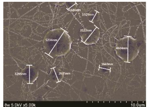
Figure 6. Micro-spheres ranging from 1,669 nm to 5,234 nm. The spinning solution used here is 8 wt.% Polylactide (PLA) with molecular weight of M_w \approx 100000 , dimethylformamide (DMF) is used as a solvent. The applied voltage is 15 kV and the distance between the solution surface and the metal receiver is 15cm
