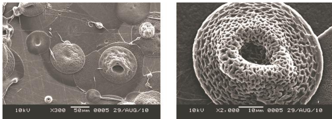
Figure 14. SEM images of the porous PBST electrospun mat with the voltage supplied 20 kV
