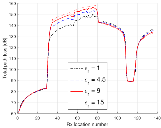
FIGURE 9. Path loss at different MT positions for \epsilon_r = 1, 4.5, 9, and 15 for the UMI configuration. \sigma = 0.09 S/m. Diffraction model: UTD.
