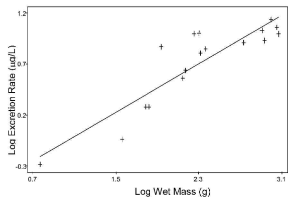
Fig. 3. Relation between wet fish biomass and excretion of ammonium ( \mu\text{g/L} ).
