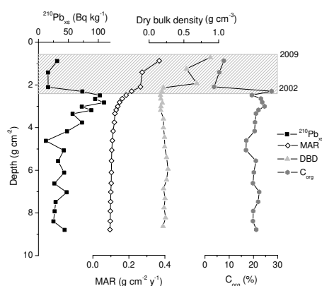
Figure B1. ^{210}\text{Pb}_{\text{XS}} , mass sedimentation rates (MAR), dry bulk density and C_{\text{org}} content in a mangrove sediment core at the Everglades, Florida. The gridded area represents the period 2002–2009, when Hurricane Wilma (2005) delivered a large pulse of sediment (Adapted from Smoak et al., 2013).
