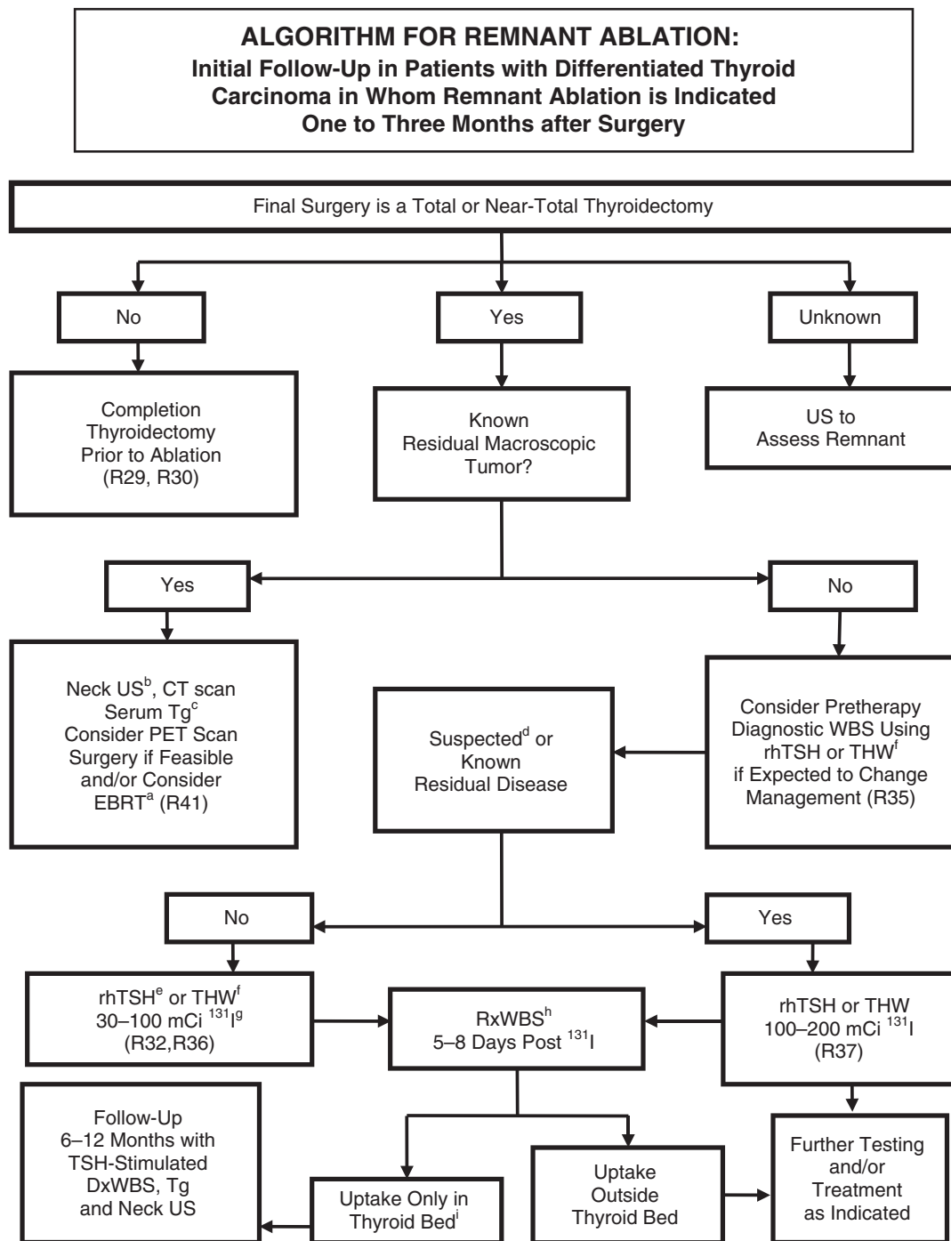
FIG. 3. Algorithm for initial follow-up of patients with differentiated thyroid carcinoma.
