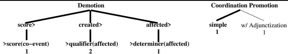
Figure 5.13: Demotion and Promotion revision operation hierarchy
