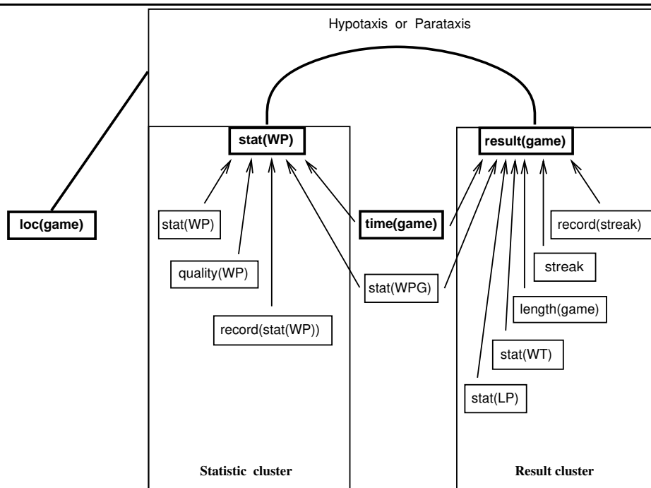
Figure 2.5: Concept clusters
