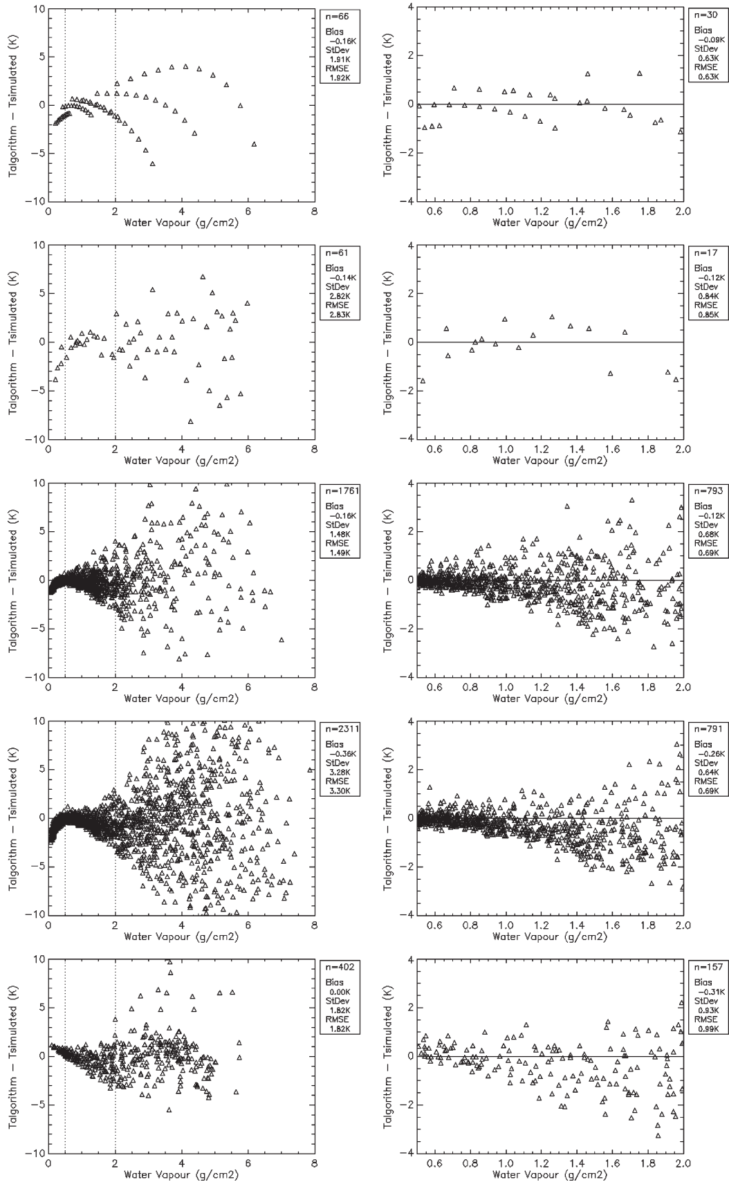
Fig. 5. Test of the SC algorithm using the same simulated data than used for retrieving the AFs. Plots show the difference between the LST retrieved with the SC algorithm ( T_{algorithm} ) and the one included in the simulated database ( T_{simulated} ) (left column) for the whole range of water vapor values and (right column) only for the range between 0.5 and 2 g \cdot cm^{-2} . Values of bias, standard deviation, and rmse are also given. Surface emissivity has been assumed to be 1.0. From top to bottom, plots correspond to STD66, TIGR61, TIGR1761, TIGR2311, and SAFREE402 databases.
