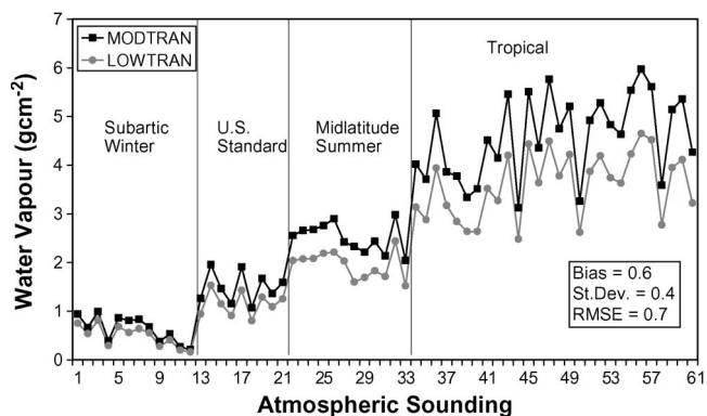
Fig. 4. Output atmospheric water vapor content from LOWTRAN and MODTRAN for each atmospheric profile included in the TIGR61 database. Model atmosphere in which each atmospheric sounding is assigned is also shown.
