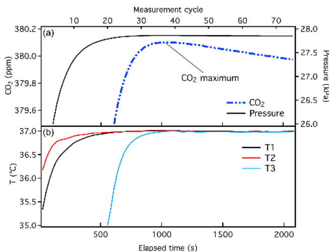
Figure 2. Typical data from a manometric run, showing the small volume pressure and CO 2 (+N 2 O) calculated as a function of time (a), and temperature measured at three locations within the oven (b). Historical manometric records are time-stamped with “measurement cycle”, which is shown on the upper x axis. Here, each measurement cycle corresponds to \sim 30 s. Temperature probe T3 is adjacent to the small volume and is cooled to liquid nitrogen temperature during extraction.
