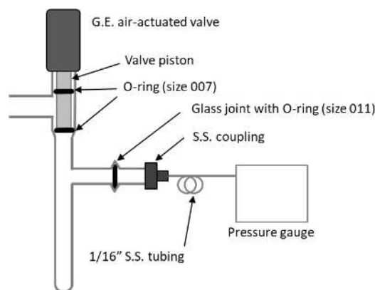
Figure 3. Diagram of the small volume showing position of Viton O-rings in the air-actuated valve (Glass Expansion, Pocasset, MA) and a glass joint.
