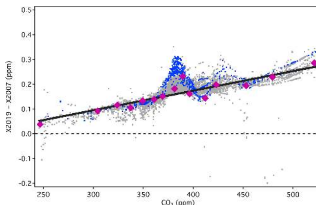
Figure 13. Differences between X2019 and X2007 tertiary assignments from 1995 to 2017 (NDIR only), showing 2008 analysis in blue and all others in gray. A linear scale conversion derived from primary standards (pink) is shown as the black line.
