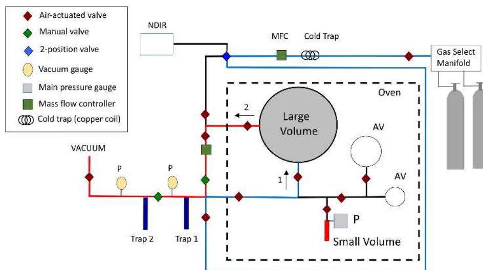
Figure 1. Schematic of the NOAA manometer. Air is passed through a cold trap ( \sim -69^\circ\text{C} ) and mass flow controller into the large volume in the direction of arrow (1), which is shown as blue lines. After the temperature and pressure of the air in the large volume are recorded, the air is drawn from the large volume in the direction of arrow (2) (red lines) and through traps 1 and 2 to cryogenically trap the CO 2 . The CO 2 is cryogenically purified in glass traps 1 and 2 and then transferred to the small volume where its pressure and temperature are determined. Auxiliary volumes (AVs) are used in separate experiments to determine the ratio of large and small volumes (volume ratio). The dashed line depicts a temperature-controlled oven housing the glass volumes and pressure gauge.
