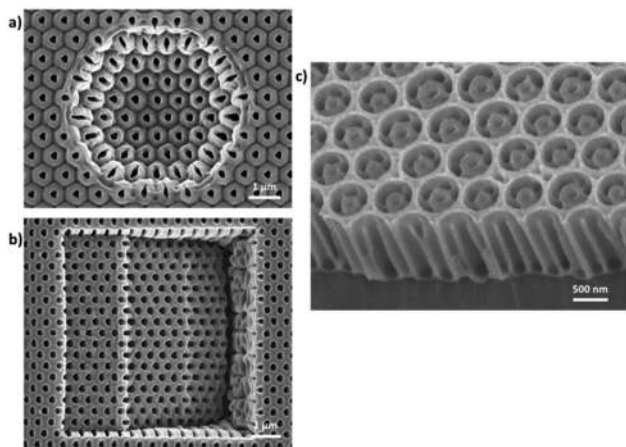
Fig. 16 (a) and (b) SEM images of anodized nanopore arrays across (a) hemispheric-shaped aluminium surface and (b) stair-case shaped surface. The inter-pore distance between the nanopores is 350 nm and 200 nm, respectively. Reprinted with permission from ref. 181. Copyright © 2011 Elsevier Ltd. (c) SEM image of a hierarchical AAO structure by NSL technique. The period of the pre-patterned aluminium substrate is 680 nm. Reprinted with permission from ref. 198. Copyright © 2012 WILEY-VCH Verlag GmbH & Co. KGaA, Weinheim.
