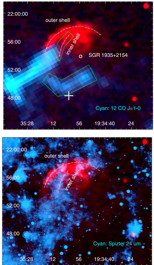
Figure 3. Composite images comparing the THOR 1.4 GHz radio continuum (red) and PMO ^{12}\text{CO } J = 1-0 (upper panel, cyan color; V_{\text{LSR}} = 28-32 \text{ km s}^{-1} ) or Spitzer 24 \mu\text{m} (lower panel, cyan color) emission. The polygons in the upper panel define the regions “inner shell” and “arc” for CO spectral extraction. The circle and cross signs denote the position of the magnetar and 1720 MHz OH maser.
