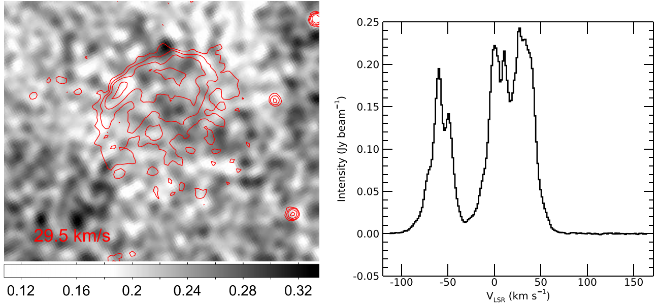
Figure 12. Left: H I morphology at 29.5 \text{ km s}^{-1} . The unit of the color bars is \text{Jy beam}^{-1} . Right: averaged H I spectrum extracted from the SNR with a radius of 5/5 .
