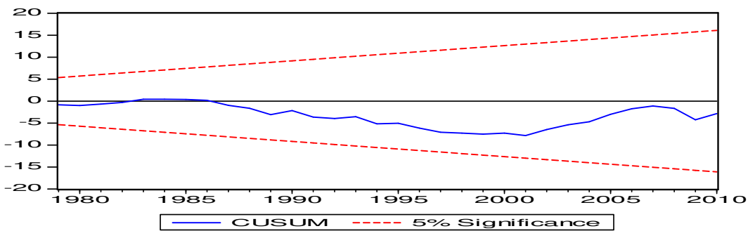
Figure 1. Plot of Cumulative Sum of Recursive Residuals
