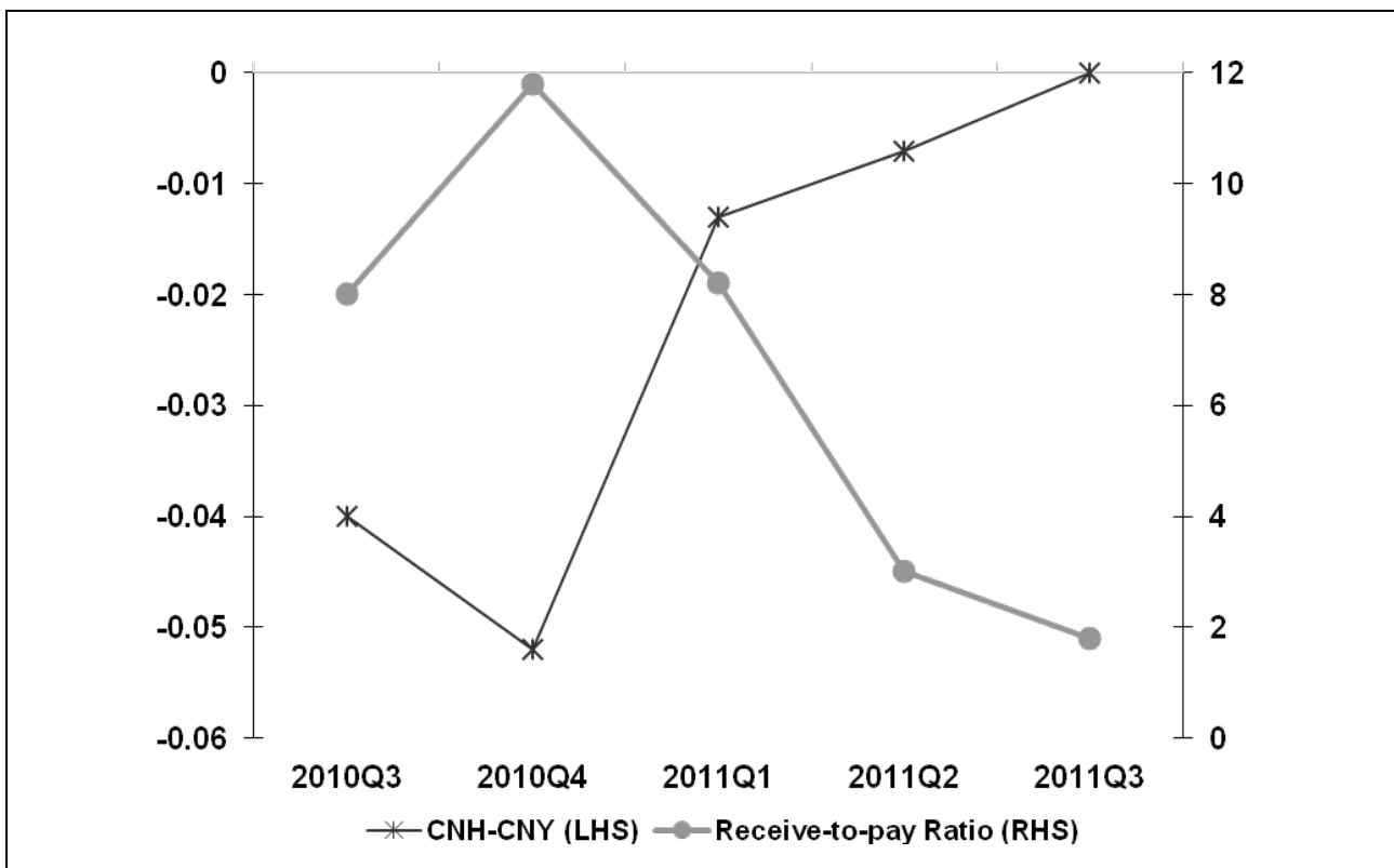
Figure 3: Correlation Between CNH–CHY Spread and Yuan Import–Export Settlement Ratio
