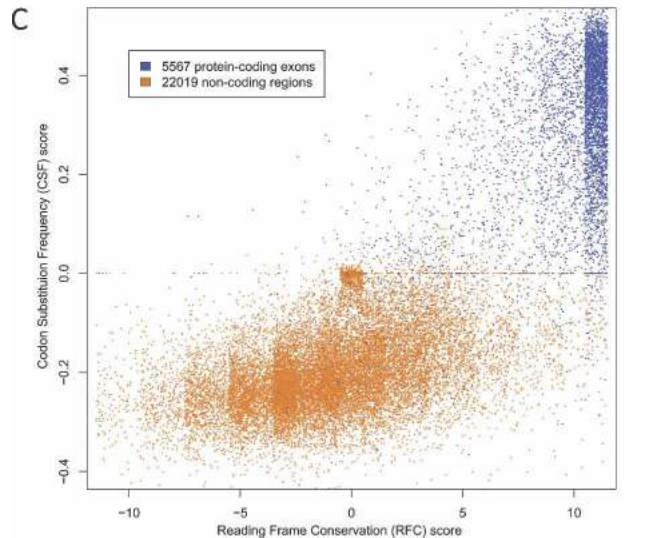
Figure 1. Evolutionary signatures for protein-coding gene identification. (A) Within coding regions, triplet substitutions are biased toward conservative codon substitutions (Codon Substitution Frequencies, CSF). Additionally, indels in coding regions are strongly biased to be a multiple of three in length (reading frame conservation; RFC). (B) The color of each codon substitution between the D. melanogaster sequence and an informant sequence corresponds to a log-odds score of observing that substitution in a coding region versus a noncoding region. (C) Quantitative metrics of RFC and CSF distinguish coding and noncoding regions. Shown in blue are 5567 coding exons of well-studied genes and in orange are 22,019 regions chosen uniformly at random from the noncoding part of the genome, with the same length distribution as the exons. The CSF score is length-normalized and the discrete RFC score is dithered by adding random noise uniformly from (-0.5, 0.5) for the purposes of visualization.
