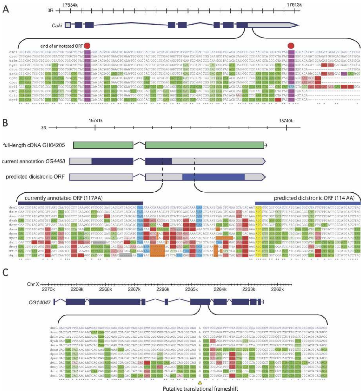
Figure 5. Unusual protein-coding structures identified by evolutionary signatures. (A) A well-conserved 30-aa ORF immediately following the stop codon in the gene Caki suggests translational readthrough. Note the perfect conservation of the putative readthrough stop codon, the “wobble” of the downstream stop codon, and the precipitous loss of conservation following the downstream stop codon, typical of a true translation stop. (B) A well-conserved ORF within the annotated 3' UTR of CG4468 suggests a dicistronic transcript structure. Note the region of poor conservation that extends precisely from the upstream stop codon to the downstream start codon, suggesting separate translation of the two ORFs. (C) An abrupt change in the reading frame upon which selection appears to act within an exon of CG14047 is suggestive of a “programmed” translational frameshift (see also Supplemental Fig. 2).
