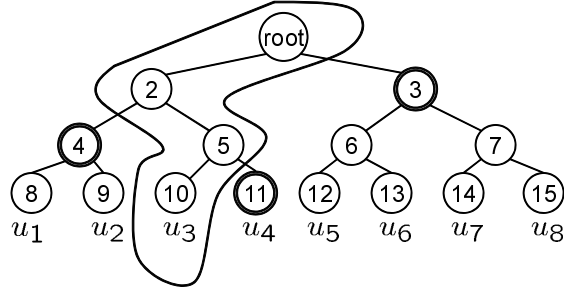
Fig. 1. Example of KUNode
