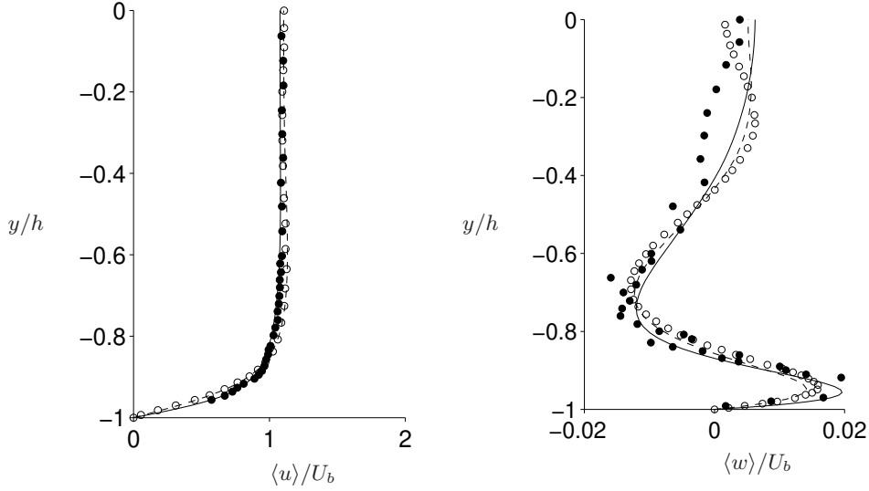
FIGURE 2. Mean velocity components at z/h = -0.7 : streamwise component (left), cross stream component (right). Present DNS results (— Re_b = 3500 --- Re_b = 2205 ) compared to reference DNS data ( \circ ) and experimental data ( \bullet ).
