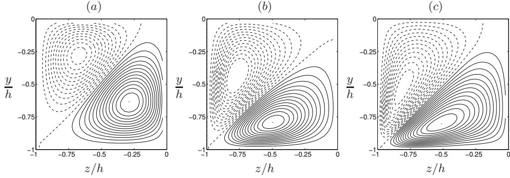
FIGURE 9. Streamlines \langle\psi\rangle(y, z) of secondary mean flow computed using \langle v\rangle and \langle w\rangle averaged over all quadrants (with increment [\max\langle\psi\rangle - \min\langle\psi\rangle]/30 ). Dashed lines correspond to clockwise rotation, continuous lines to counterclockwise motion. (a) Re_b = 1077 ; (b) Re_b = 2205 and (c) Re_b = 3500 . Only [-1, 0] \times [-1, 0] quadrant shown.
