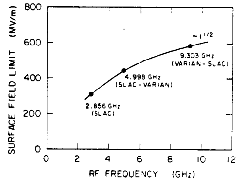
Fig. 1. Peak breakdown surface fields measured as a function of frequency.
