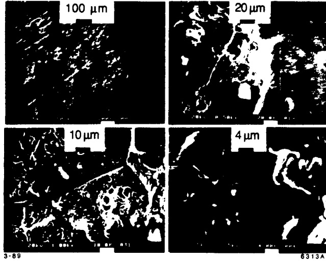
Fig. 4. Scanning electron microscope pictures of S-band, \pi -mode two-cavity nose cone showing RF breakdown damage (note different scales in microns).
