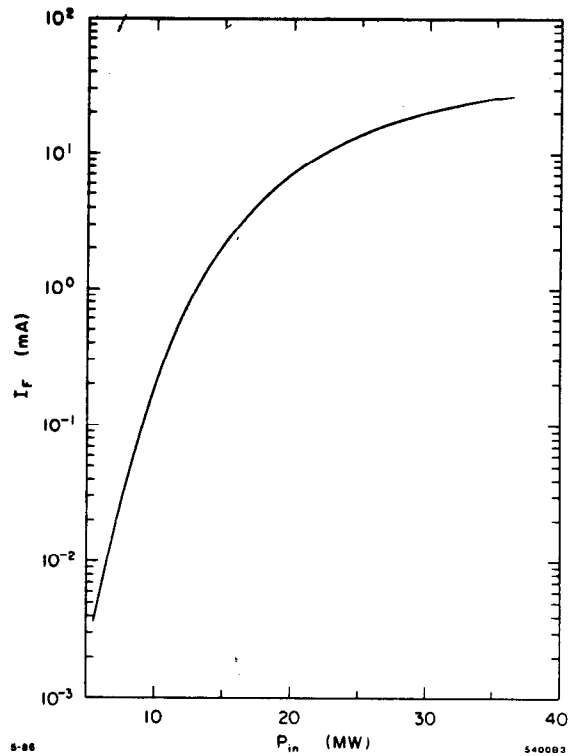
Fig. 14. Field emitted current transmitted through downstream window (right-hand side in Fig. 6) to Faraday cup, as a function of peak input power.
