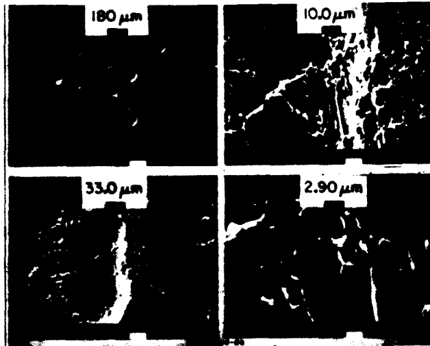
Fig. 18. Scanning electron microscope pictures of C-band cavity nose cone showing RF breakdown damage (note four successive scales in microns).
