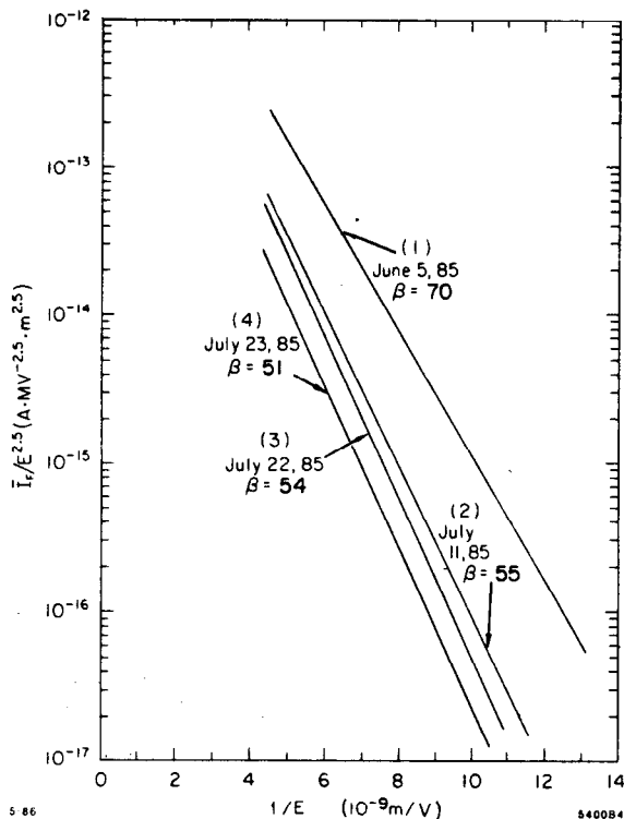
Fig. 19. RF Fowler-Nordheim plots for S-band (seven-cavity, 2\pi/3 -mode) structure as a function of time. Curve (4) was recorded shortly after argon scrubbing and pumpdown.
