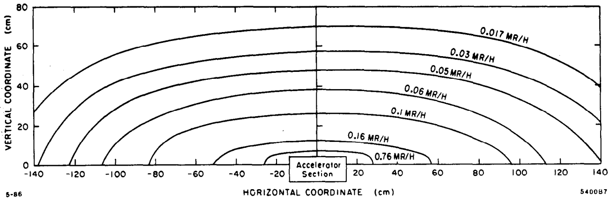
Fig. 16. Average x-ray dosage distribution around S-band (seven-cavity, 2\pi/3 -mode) accelerator section (300 MV/m surface field, 2.5 \mu sec, 120 pps).
