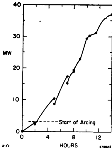
Fig. 11. Typical RF processing schedule for S-band, seven-cavity structure.
