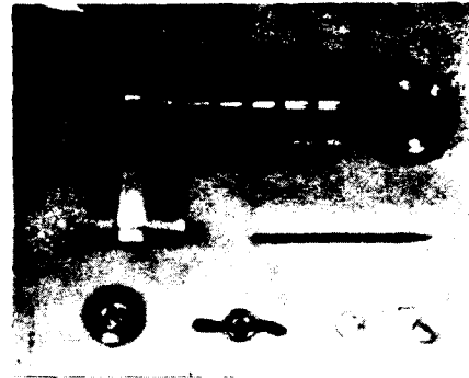
Fig. 1. Collection of S-band (seven-cavity, 2\pi/3 -mode), C-band and X-band cavities used in tests.
