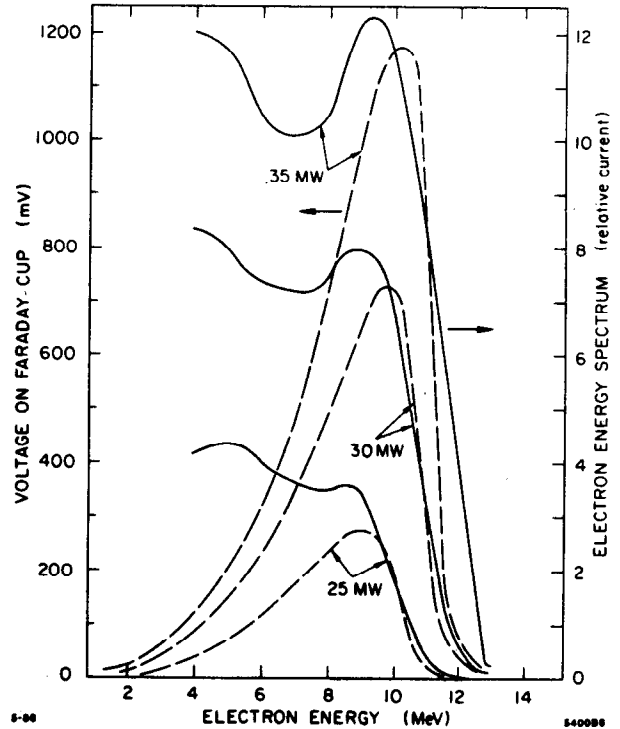
Fig. 15. Uncorrected (dashed lines) and corrected (continuous lines) electron energy spectra for various values of peak input power into S-band seven-cavity structure.
