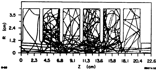
Fig. 13. Typical field emitted electron trajectories plotted for S-band ( 2\pi/3 -mode) structure by means of computer program NEWTRAJ (courtesy of R. Parodi).
