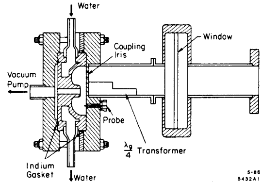
Fig. 4. Cross-sectional view of demountable C-band cavity.
