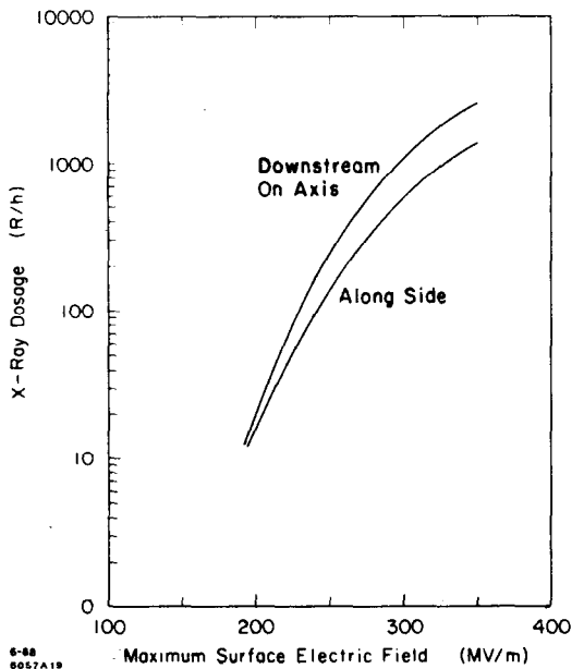
Fig. 17. Average x-ray dosage around S-band (two-cavity, \pi -mode) accelerator section (2.5 \mu sec, 60 pps) as a function of peak field.
