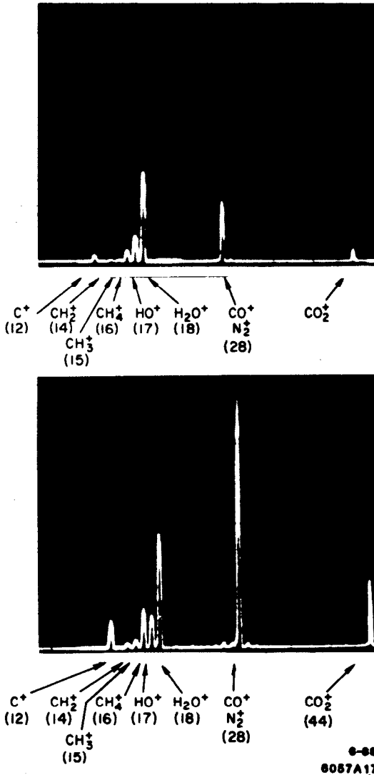
Fig. 8. Residual gas analyzer displays during RF processing of S-band, two-cavity structure, a) before breakdown, and b) immediately after breakdown.
