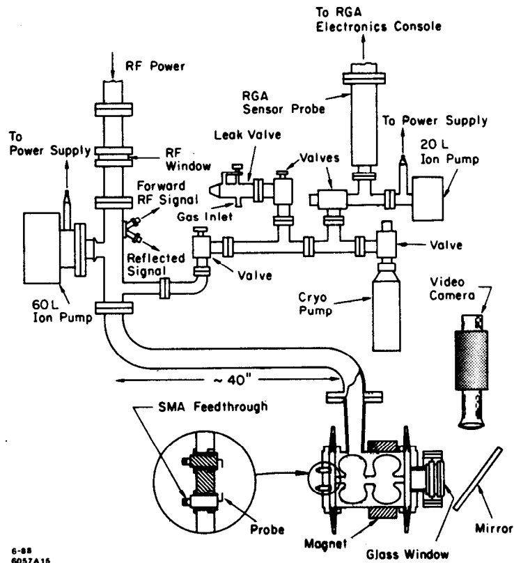
Fig. 7. Experimental set-up used for S-band (two-cavity, \pi -mode) structure, showing details of vacuum system.
