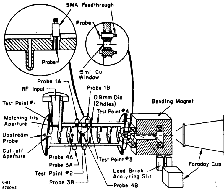
Fig. 6. Experimental set-up used for S-band (seven-cavity, 2\pi/3 -mode) structure.
