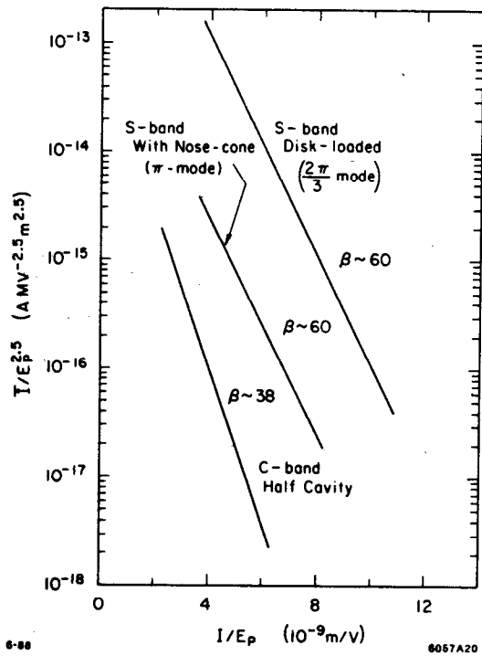
Fig. 12. Fowler-Nordheim plots for S-band and C-band structures.
