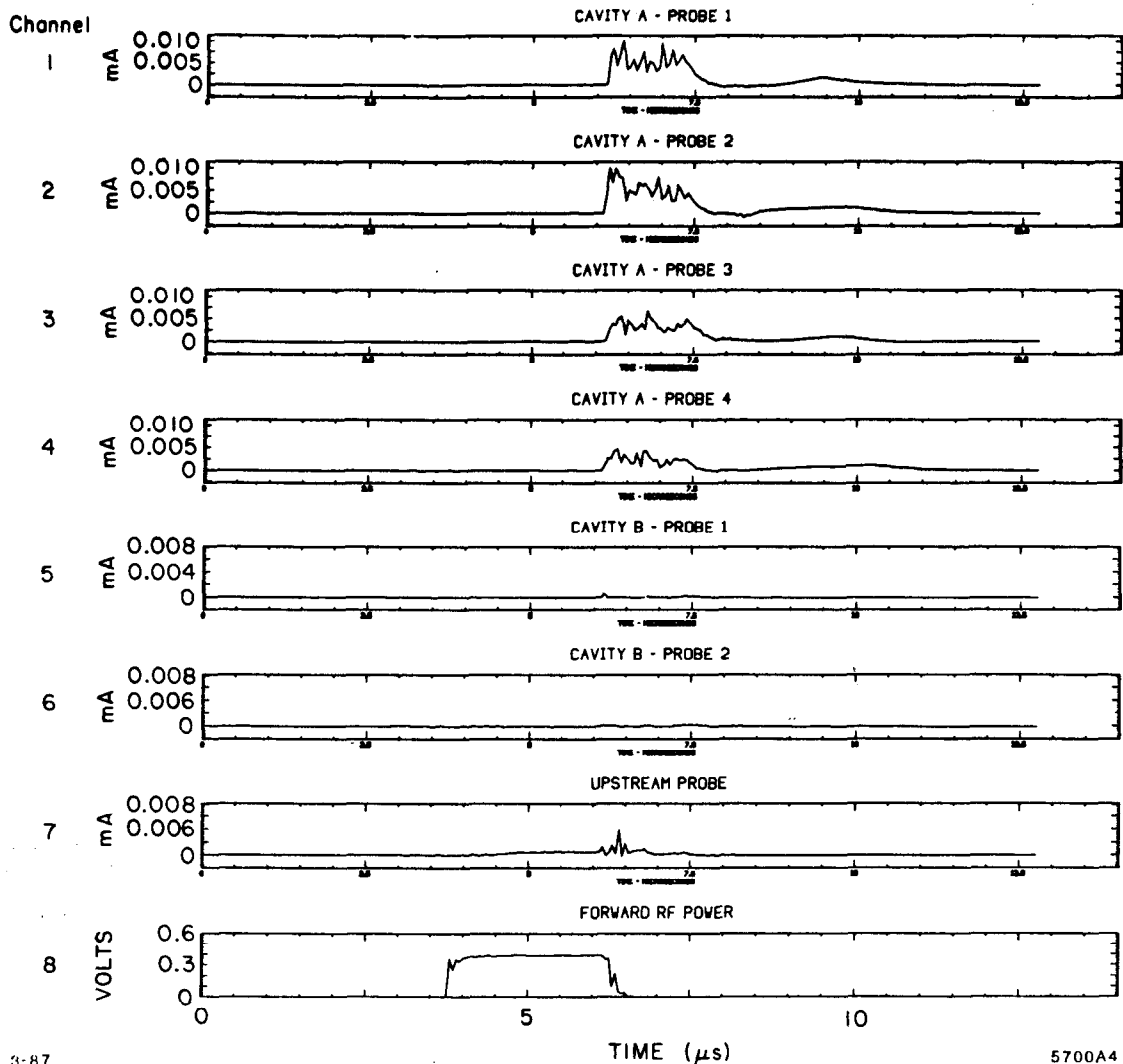
Fig. 10. Breakdown "event" recorded at four radial probes in full-field cavity (A), two radial probes in half-field cavity (B), and one upstream probe. The forward RF pulse provides a time reference.
