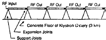
Fig. 1: The MDL runs the accelerator length in the klystron gallery. RF is distributed to the local RF distribution system in each sector, where timing information is extracted, and frequency is increased by a factor of 6. Attachment to gallery floor helps decrease temperature dependence by constraining the physical line length.
