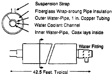
Fig. 4: Detail of the PRL insulation package. Each line segment consists of a length of temperature-stable 1/2-inch semirigid foam Heliax, surrounded by a water jacket and conventional water line insulation. Lines are suspended on cables to decouple changes in building length due to ambient temperature changes from phase length of reference line.
