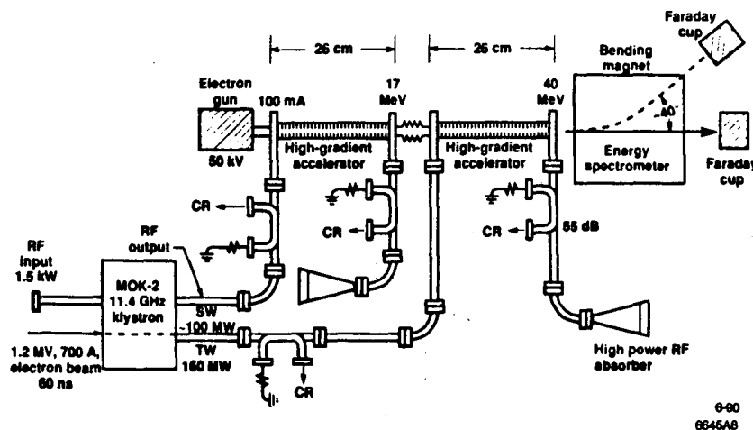
Figure 1: High gradient two-stage accelerator test.
