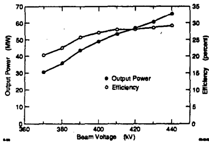
Figure 3: Measured output power vs. beam voltage for klystron.
