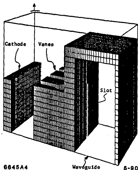
Figure 7: Simulation of waveguide-coupled anode circuit.
