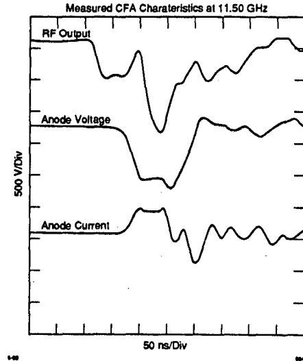
Figure 6: Measured CFA characteristics at 11.5 GHz.
