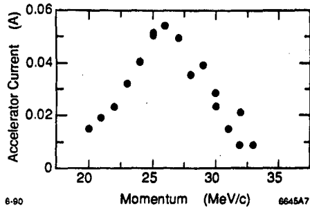
Figure 2: Energy spectrum of two-stage accelerated beam.
