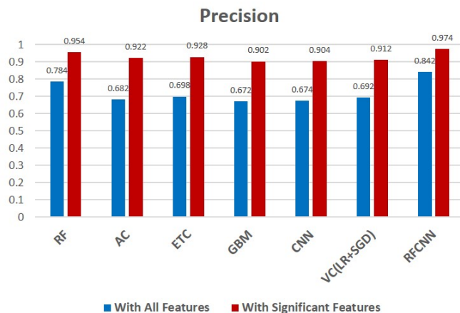
FIGURE 7: Precision of all Ensemble learning models.
