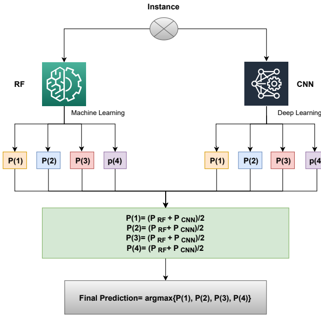
FIGURE 4: Architecture of the proposed RFCNN.
