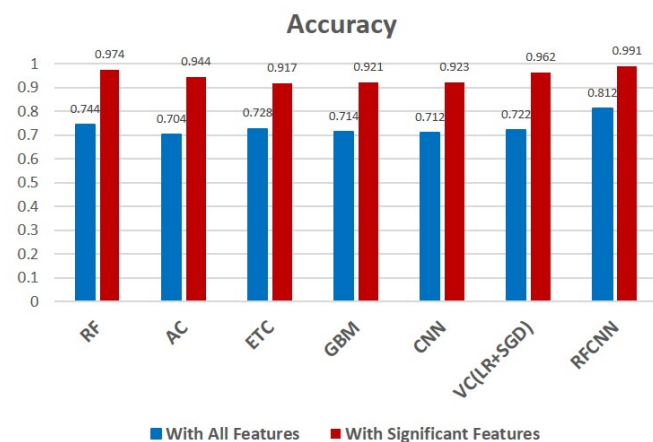
FIGURE 6: Accuracy of all Ensemble learning models.
