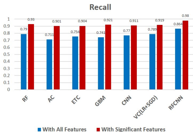
FIGURE 8: Recall of all Ensemble learning models.
