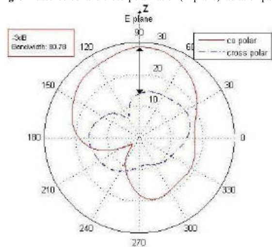
Fig. 7 Measured co- and cross-polarization (E-plane) radiation pattern
