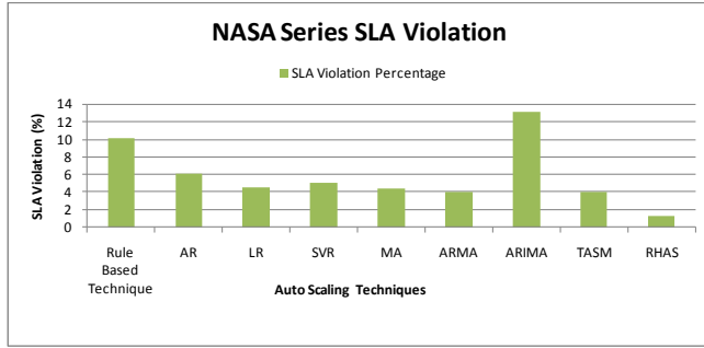
Fig. 19 NASA series SLA violation
