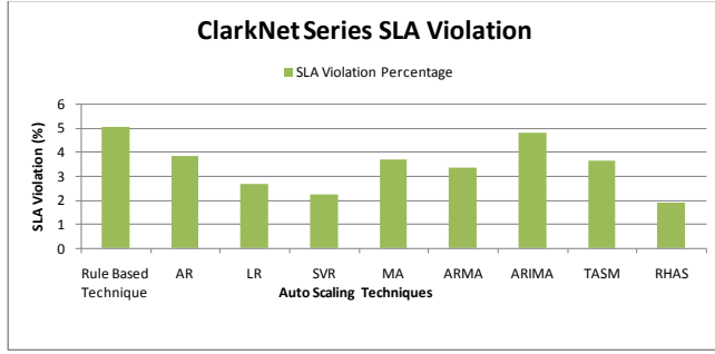
Fig. 18 ClarkNet series SLA violation
