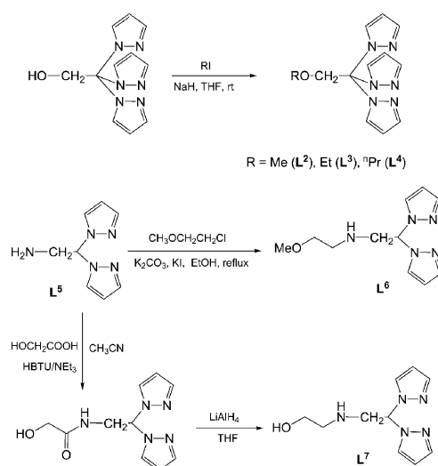
Scheme 1 Synthesis of the pyrazole-based ligands.
