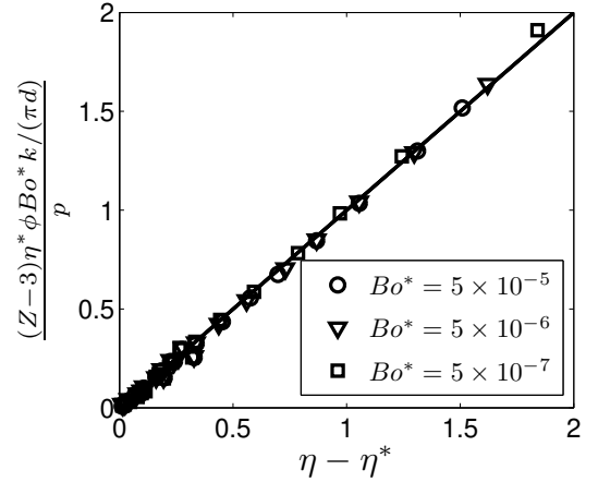
FIG. 13. Predictions of C_{\text{Rumpf}}^{\text{corr}}/p taking account of non-affine displacements versus \eta - \eta^* from simulation results for different volume fractions ( 0.50 \leq \phi \leq \phi_c ), cohesion levels (as shown in the legend), and friction coefficients ( \mu = 0.1, 0.3, \text{ and } 0.5 ) in the cohesive regime. In all cases, Hookean contact and van der Waals force model are used. The line represents y = x .
