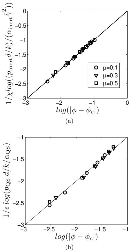
FIG. 6. Collapse of pressure for (a) inertial regime and (b) quasistatic regime. For both (a) and (b), the solid line has a slope of 1 and y -intercept of 0. All points with different volume fractions and particle friction coefficients fall on the lines. Hookean contact is used.
