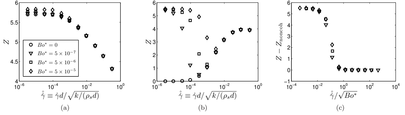
FIG. 3. The average coordination number versus scaled shear rate at \mu = 0.1 and various modified Bond numbers for (a) \phi = 0.62 and (b) \phi = 0.59 . In (c), the data from (b) are collapsed into one curve by subtracting Z for non-cohesive system from that of cohesive systems and rescaling the shear rate. Hookean contact and van der Waals force model are used here.
