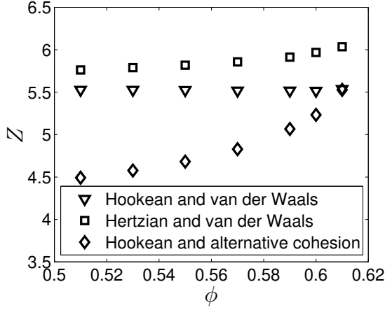
FIG. 14. The average coordination number versus volume fraction in the cohesive regime for particles with \mu = 0.1 and Bo^* = 5 \times 10^{-5} .
