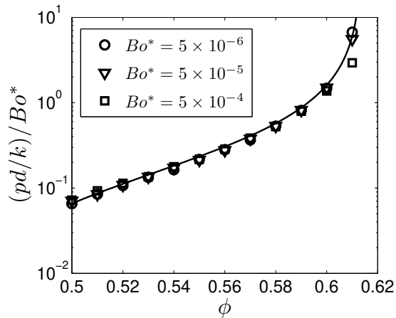
FIG. 10. Dimensionless pressure scaled by Bo^* versus volume fraction in the cohesive regime at \hat{\gamma} = 3.2 \times 10^{-6} for \mu = 0.1 and various Bo^* values. The line represents 0.15 \frac{|\phi - \phi_a|}{|\phi_c - \phi|} , where \phi_c(\mu = 0.1) = 0.614 and \phi_a(\mu = 0.1) = 0.45 . Hookean contact and van der Waals force model are used here.
