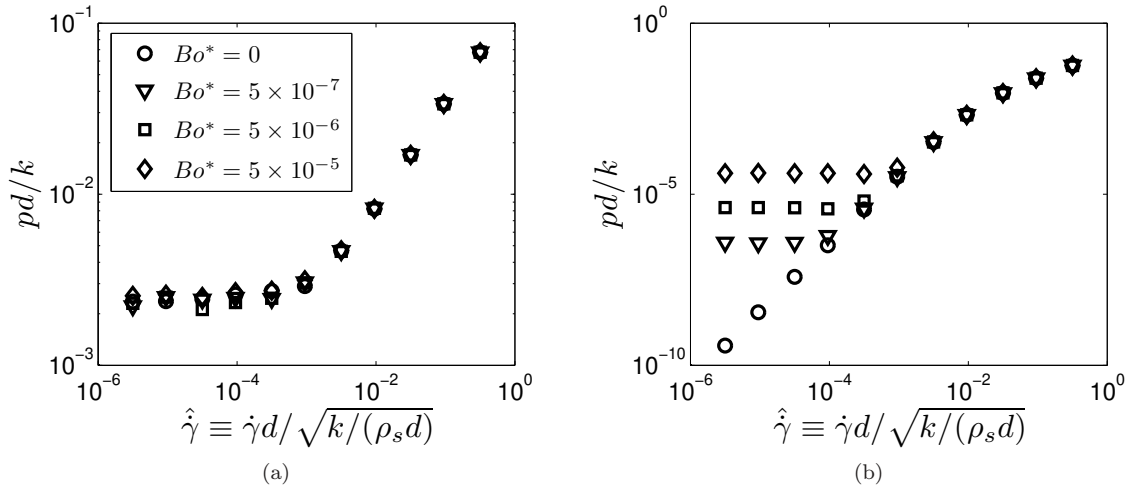
FIG. 4. Scaled pressure versus scaled shear rate at \mu = 0.1 and various modified Bond numbers for (a) \phi = 0.62 and (b) \phi = 0.59 . Hookean contact and van der Waals force model are used here.
