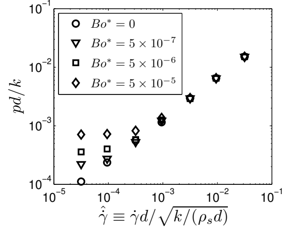
FIG. 9. Scaled pressure versus scaled shear rate at \phi = 0.614 for different cohesion levels (as shown in the legend). Inter-particle friction coefficient \mu = 0.1 is used. Hookean contact and van der Waals force model are used here.
