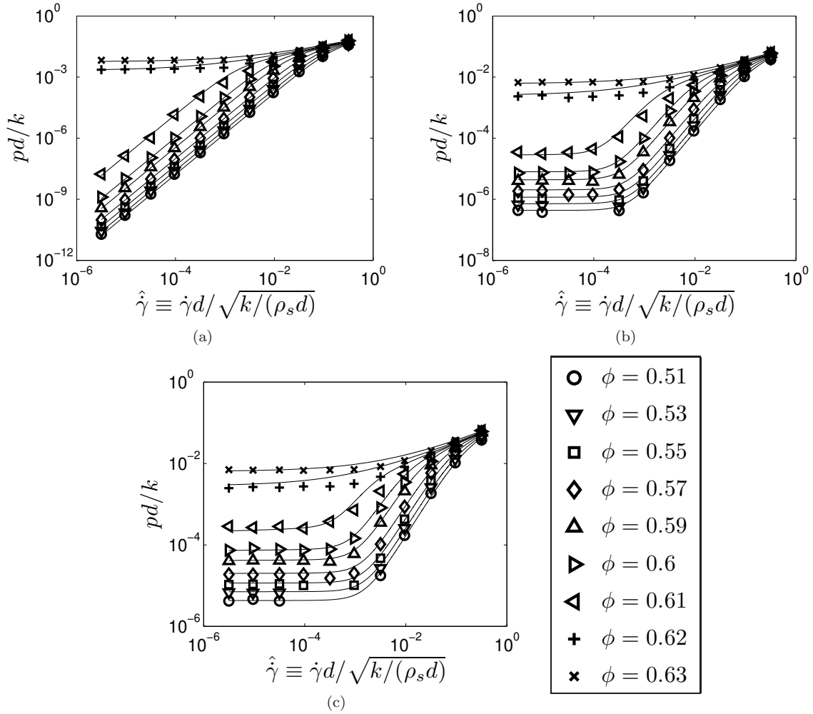
FIG. 1. Scaled pressure versus scaled shear rate for (a) non-cohesive particles, (b) cohesive particles with Bo^* = 5 \times 10^{-6} , (c) cohesive particles with Bo^* = 5 \times 10^{-5} . In all cases, Hookean contact and van der Waals force model are used, and interparticle friction coefficient \mu = 0.1 . Symbols denote simulation results, while lines denote model predictions from Eqns. (10) - (12).
