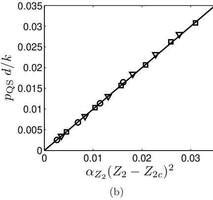
FIG. 8. Simulation data of scaled pressure in the quasistatic regime versus the predictions from the models based on (a) Z and (b) Z_2 for various volume fractions. In (a), \alpha_Z = 0.007 , and Z_c = 5.10, 4.38 , and 4.00 for \mu = 0.1, 0.3 , and 0.5 , respectively. In (b), Z_{2c} = 5.20 , \alpha_{Z_2} = 0.0077 for \mu = 0.1 ; Z_{2c} = 4.56 , \alpha_{Z_2} = 0.0083 for \mu = 0.3 ; and Z_{2c} = 4.26 , \alpha_{Z_2} = 0.0091 for \mu = 0.5 . The system is non-cohesive and Hookean contact is used. The line represents y = x .
