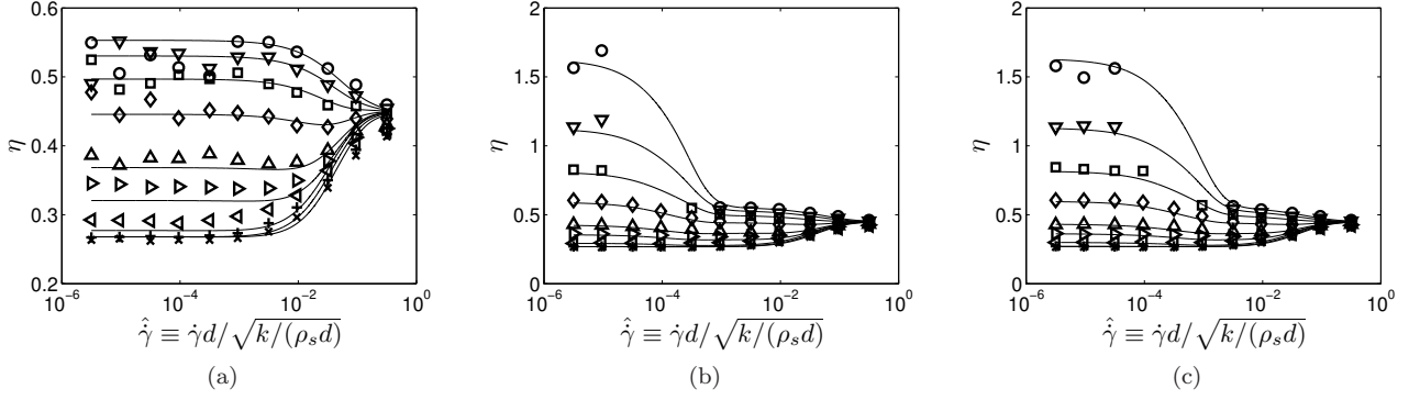
FIG. 11. Shear stress ratio versus scaled shear rate for (a) non-cohesive particles, (b) cohesive particles with Bo^* = 5 \times 10^{-6} , (c) cohesive particles with Bo^* = 5 \times 10^{-5} . In all cases, Hookean contact and van der Waals force model are used, and interparticle friction coefficient \mu = 0.1 . Symbols denote simulation results at various volume fractions as per the legend from Figure 1. Lines denote model predictions from Eqns. (13) - (15) and (19).
