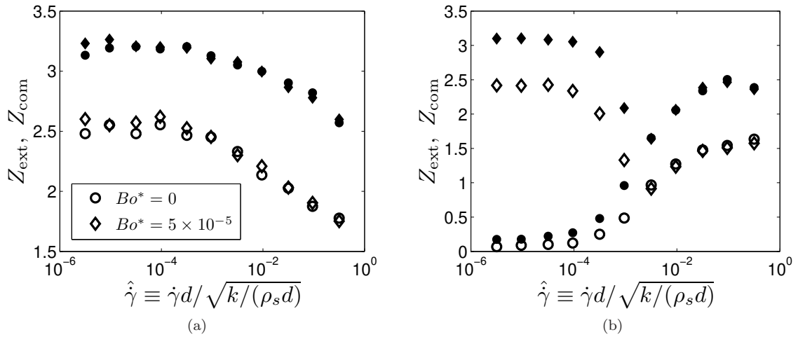
FIG. 5. The average coordination number in the extension quadrants (unfilled symbols) and compression quadrants (filled symbols) versus scaled shear rate at \mu = 0.1 for (a) \phi = 0.62 and (b) \phi = 0.59 . Hookean contact and van der Waals force model are used here.
