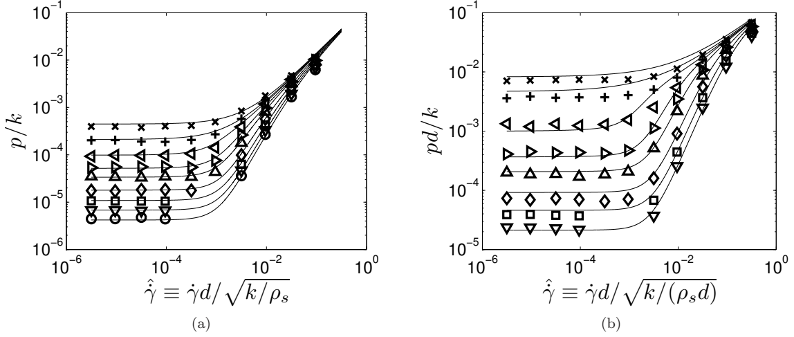
FIG. 15. Scaled pressure versus scaled shear rate for (a) Hertzian contact and the van der Waals force model, (b) Hookean contact and the alternative cohesion model [20]. Here, \mu = 0.1 and Bo^* = 5 \times 10^{-5} . Symbols denote simulation results at various volume fractions as per the legend from Figure 1. Lines denote model predictions from Eqns. (10) and (17) - (21) in (a), and Eqns. (10) - (12) in (b).
