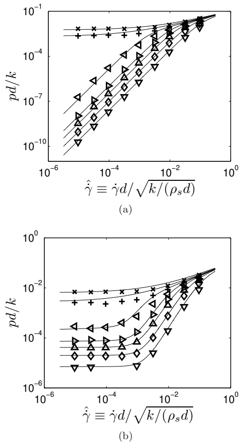
FIG. 2. Scaled pressure versus scaled shear rate for (a) non-cohesive particles, (b) cohesive particles with Bo^* = 5 \times 10^{-5} . Hookean contact and van der Waals force model are used, and interparticle friction coefficient \mu = 0.1 and restitution coefficient e = 0.02 . Symbols denote simulation results at various volume fractions as per the legend from Figure 1. Lines denote model predictions from Eqn. (7) – (12). Model parameters used are the same as those in Table I.
