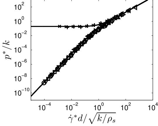
FIG. 17. Collapse of pressure versus shear rate curves for \mu = 0.1 . The pressure is scaled as p^* = p/|\phi - \phi_c|^\epsilon , and shear rate as \hat{\gamma}^* = \hat{\gamma}/|\phi - \phi_c|^{(\epsilon+\chi)/2} . \epsilon = 1.56 and \chi = 1.43 is used. Symbols denote simulation results at various volume fractions as per the legend from Figure 1. The blending function, described in Eqns. (20)–(22) and represented by solid lines, captures regime asymptotes as well as transitions. Hertzian contact with no cohesion is used.
