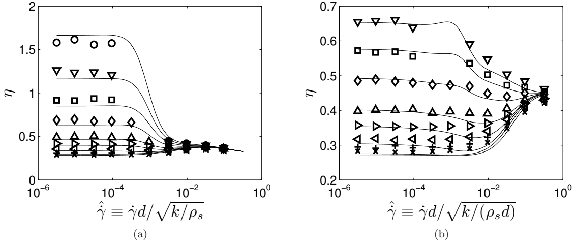
FIG. 16. Shear stress ratio versus scaled shear rate for (a) Hertzian contact and the van der Waals force model, (b) Hookean contact and the alternative cohesion model [20]. Here, \mu = 0.1 and Bo^* = 5 \times 10^{-5} . Symbols denote simulation results at various volume fractions as per the legend from Figure 1. Lines denote model predictions from Eqns. (13) - (15) and (25) in (a), and Eqns. (13) - (15) and (26) in (b).
