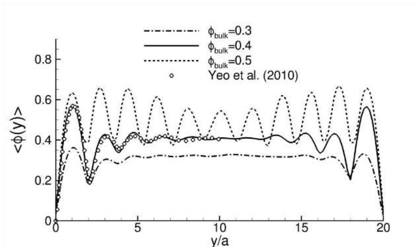
FIGURE 6. Local volume fraction \langle \phi(y) \rangle in the channel width for L_y = 20a and three bulk fractions \phi_{bulk} = (0.3, 0.4, 0.5) . Open symbols are computations by Yeo & Maxey (2010a). Particles are frictionless.
