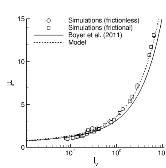
FIGURE 22. Friction coefficient \mu = \tau/\Sigma_{yy}^c as a function of I_v for frictionless ( \circ ) and frictional suspension ( \square ) simulations. Solid line is Boyer's results as represented by Eq. (4.16) with \phi_m=0.585 . Dashed line is Eq. (4.20) with \phi_m=0.64 and n=0.4 .
