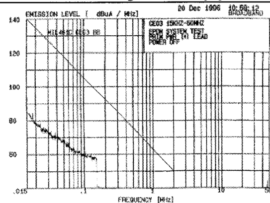
Fig. 7(a). background, broadband Fig. 7(b). Power on, broadband Fig. 7. Primary power line conducted emissions from 15 kHz to 50 MHz, CE03 (cont.)
