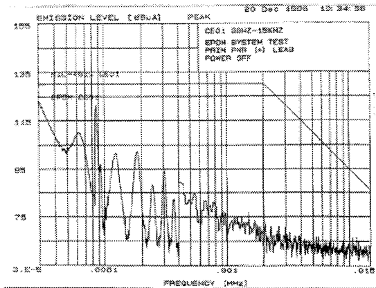
Fig. 5(a). Background Fig. 5(b). Power on Fig. 5. Primary power line conducted emissions from 30 Hz to 15 kHz, CE01
