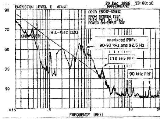
Fig. 7(d). Power on, narrowband
