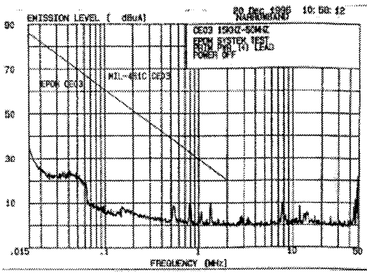
Fig. 7(c). Background, narrowband
